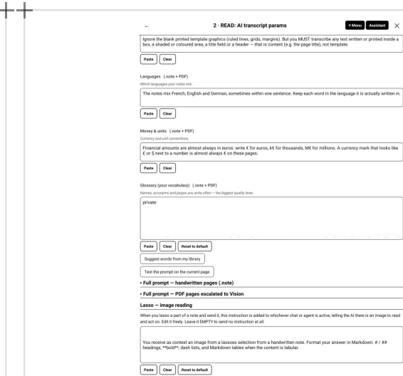
Fig. 3.3, Glossary & helpers.
