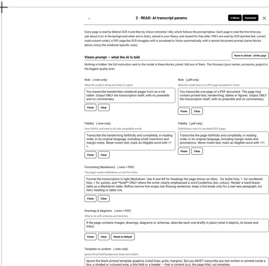
Fig. 3.2, Prompt blocks.
