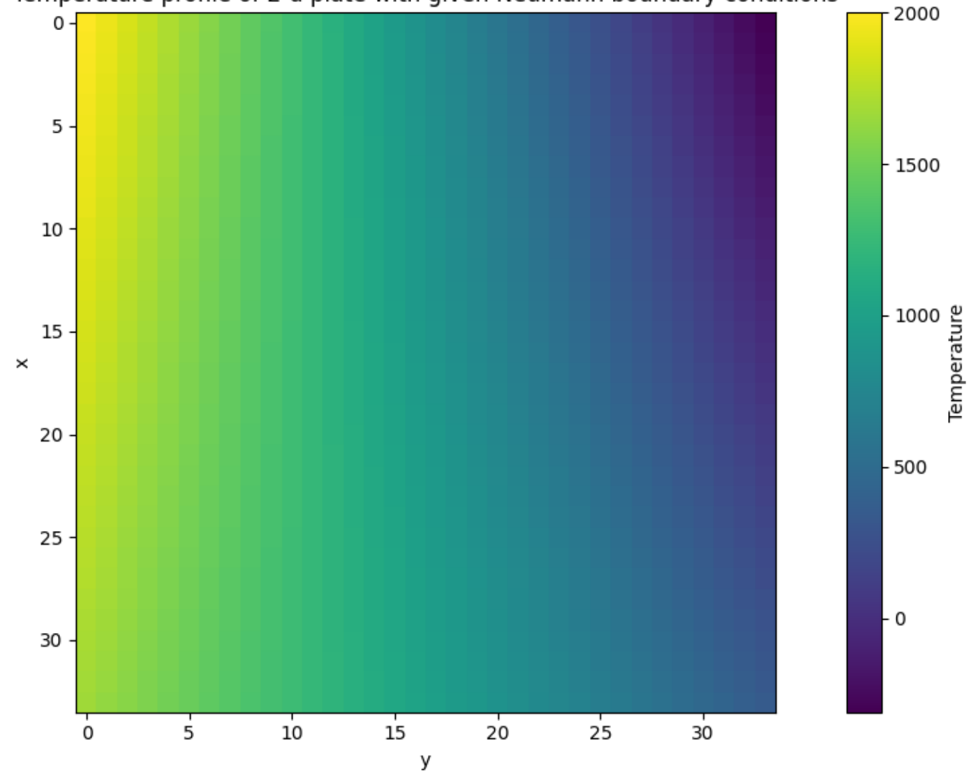
Temperature profile of 2-d plate with given Neumann boundary conditions
