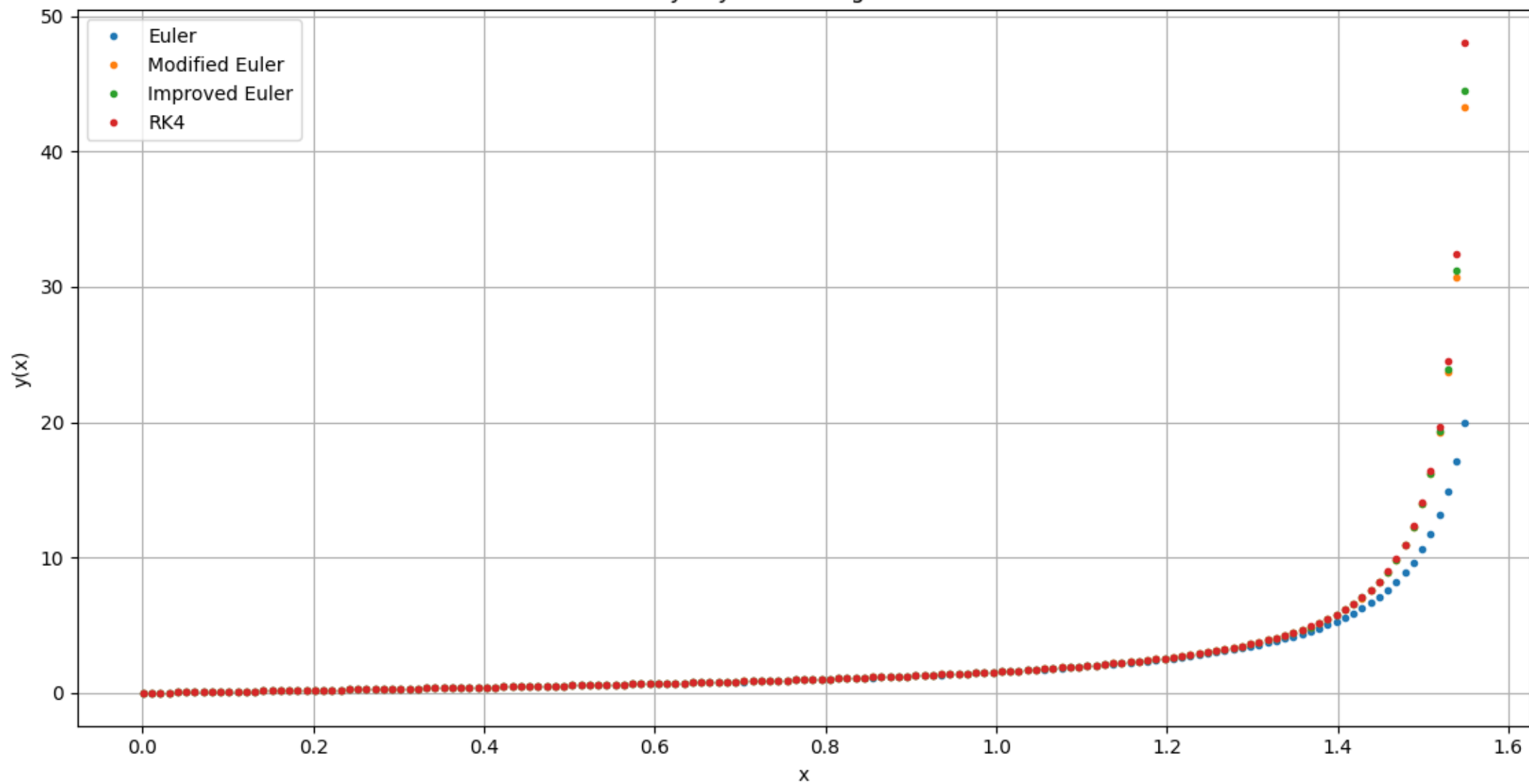
Solutions of y' = y^2 + 1 using different methods
