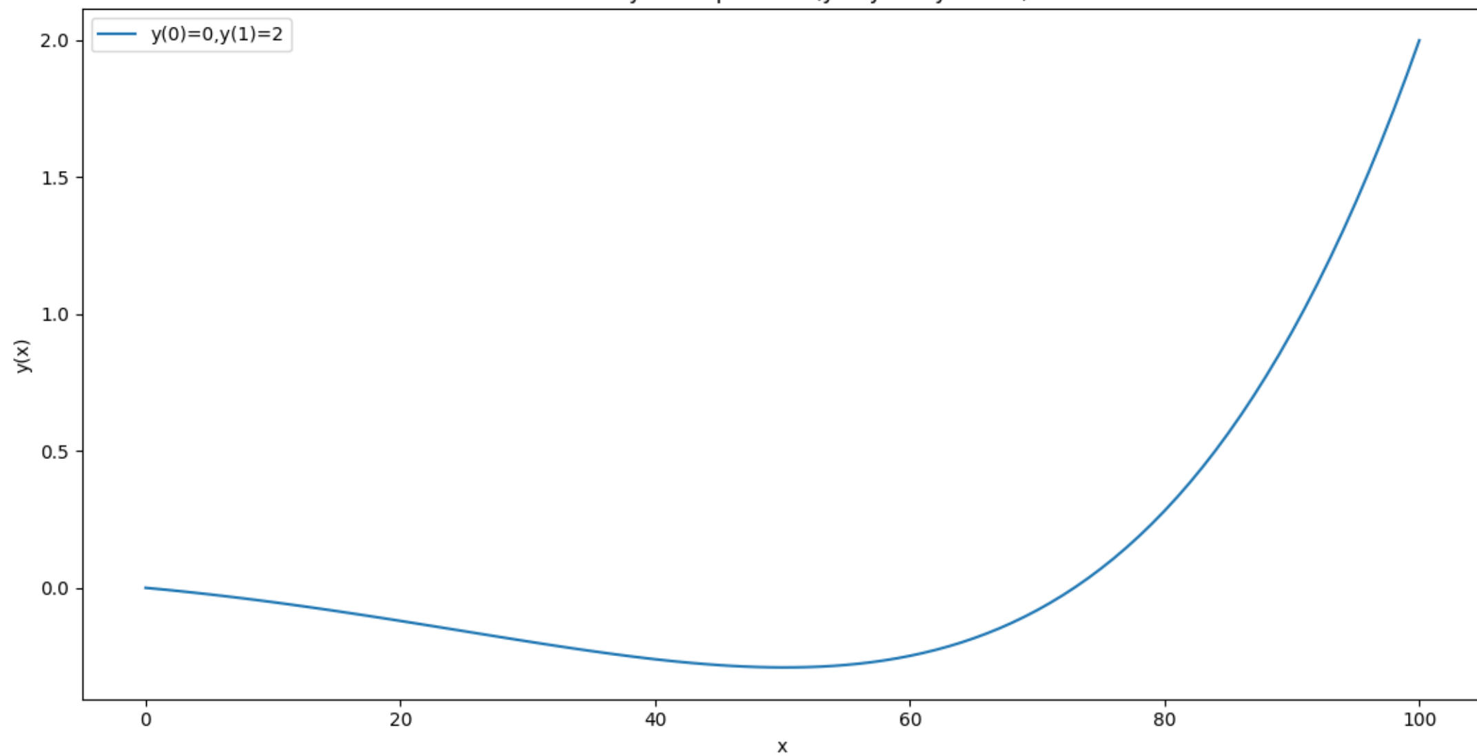
Boundary value problem ( y''-5y'+10y = 10x )
