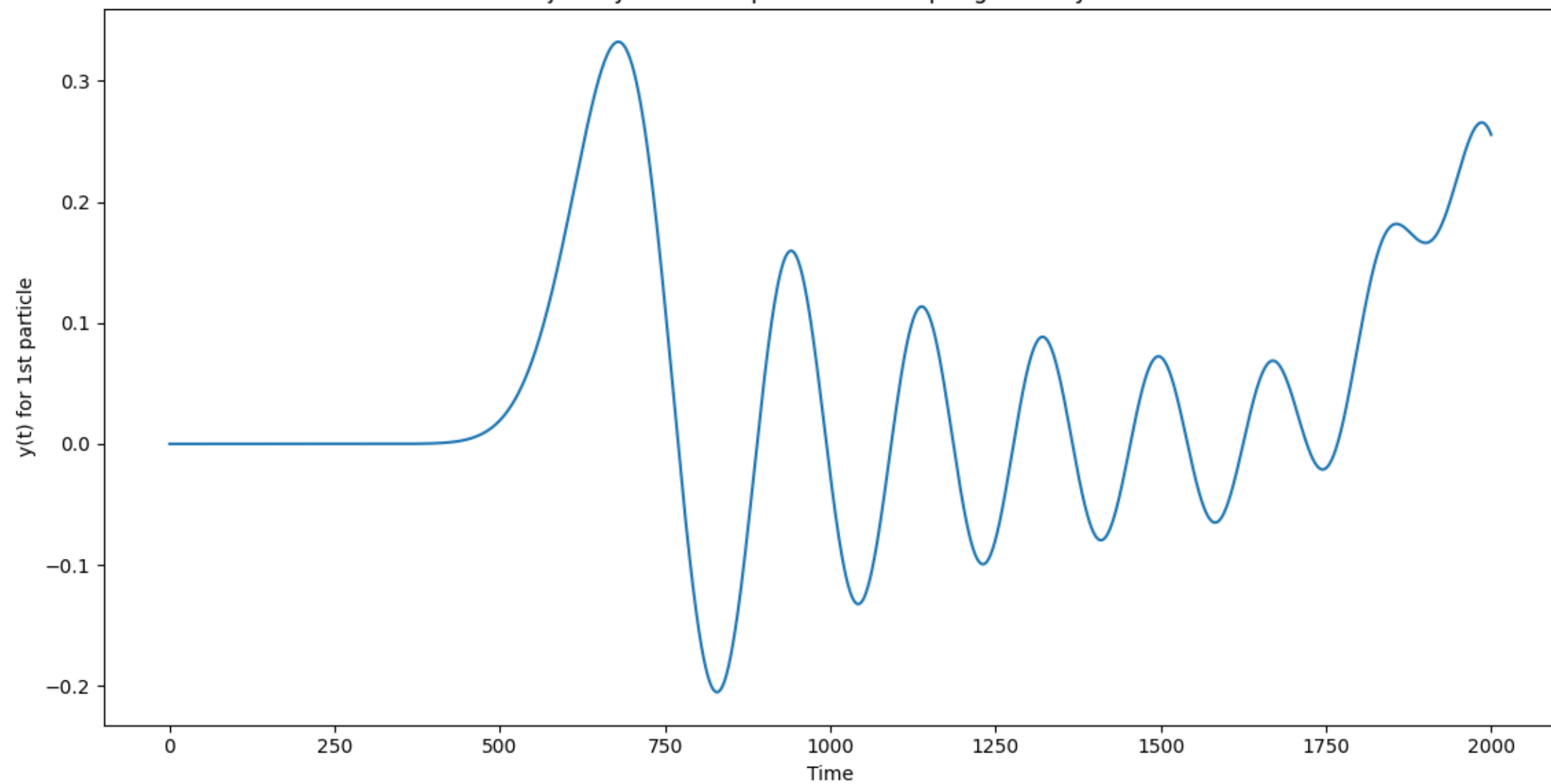
Trajectory of the 1st particle in the spring mass system
