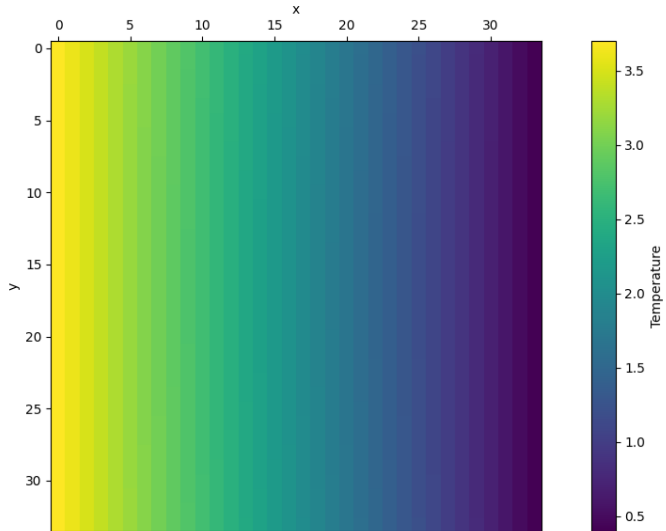
Temperature profile of 2-d plate with given boundary conditions
