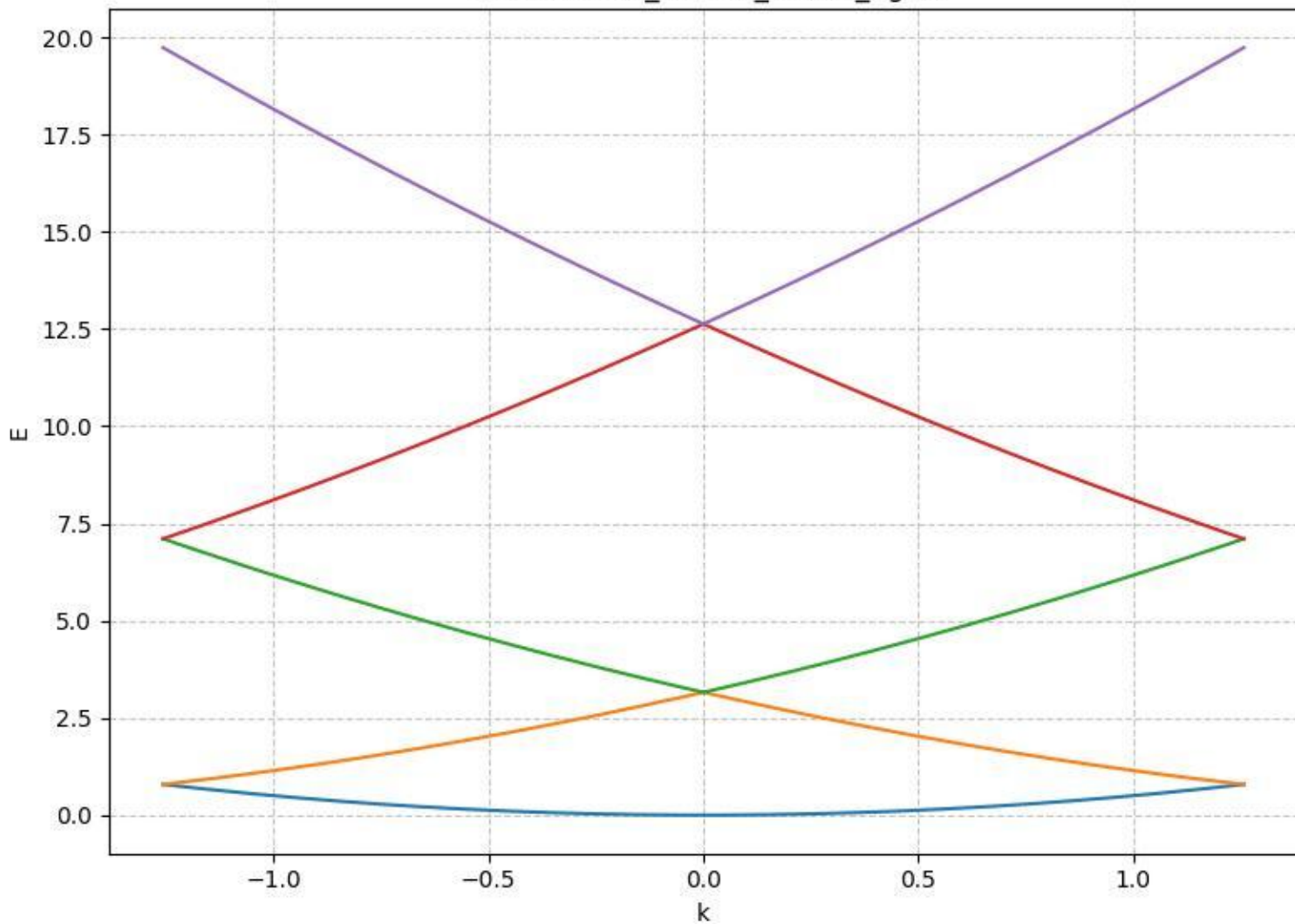
E vs k: a2.50_Vo0.00_nk401_ng11
