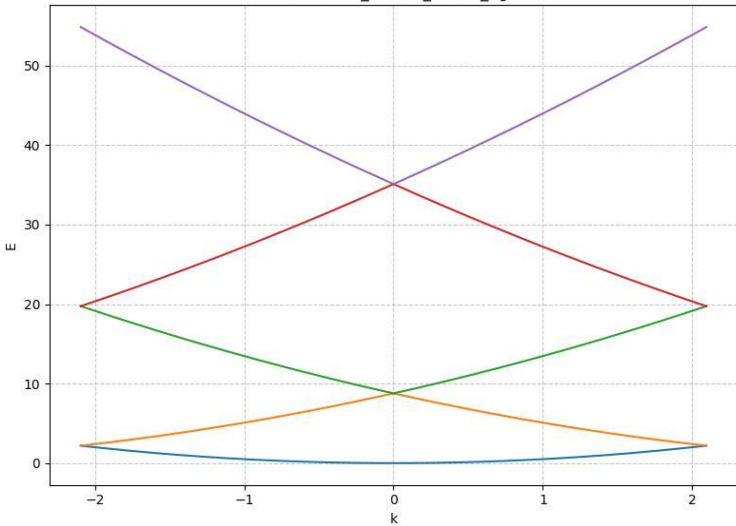
E vs k: a1.50_Vo0.00_nk401_ng11
