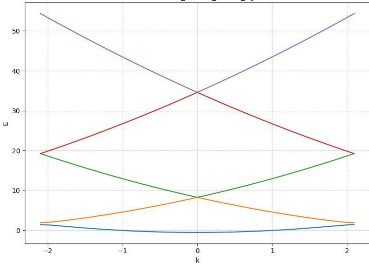
E vs k: a1.50_Vo0.50_nk401_ng11
