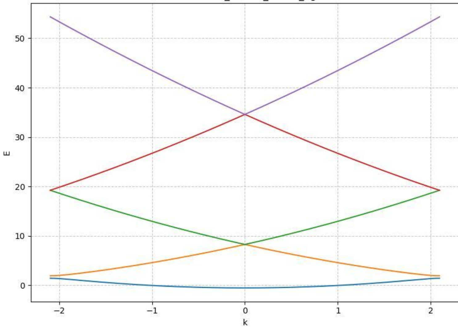
E vs k: a1.50_Vo0.50_nk401_ng61
