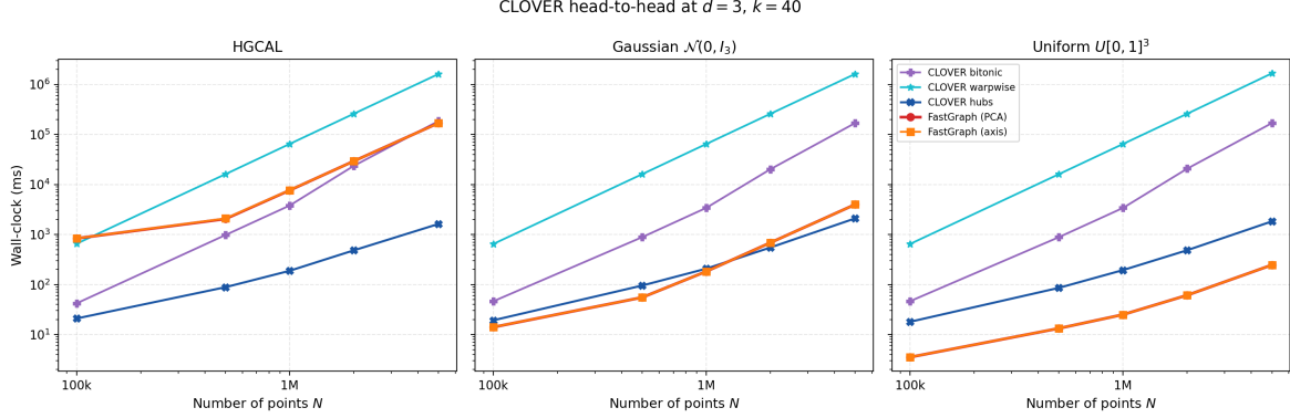
Figure 9: FastGraph vs CLOVER at d=3 , k=40 , across three data distributions: HGCAL recHits (left), synthetic Gaussian \mathcal{N}(0, I_3) (center), synthetic uniform on [0, 1]^3 (right). CLOVER’s reference implementation is hardcoded to D=3 at multiple sites ( assert(D == 3) in src/linear-scans.cu ; auto const dim = 3u in include/spatial.cuh ), so d=3 is the only dimensionality at which a direct comparison is possible.
