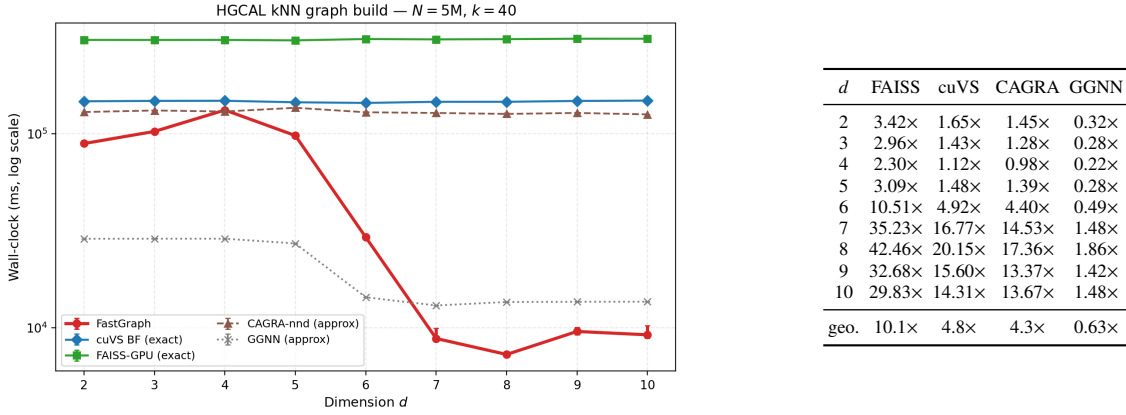
Figure 1: Headline benchmark on detector data at N=5\text{M} , k=40 . Left: dimensional scaling of wall-clock time. FastGraph is the fastest exact GPU method across the full d=2-10 range. Right: speedups of FastGraph over each backend at the same operating point. FAISS and cuVS BF are exact; CAGRA-nnd and GGNN are approximate default-recall baselines, and GGNN’s timing should be read with its substantially lower recall in this regime (Section 5.7).
