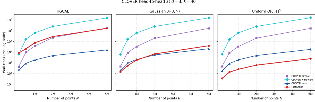
Figure 6: FastGraph vs CLOVER at d=3, k=40 , across three data distributions: HGICAL recHits (left), synthetic Gaussian \mathcal{N}(0, I_3) (center), synthetic uniform on [0, 1]^3 (right). CLOVER is only implemented for D=3 , so d=3 is the only dimensionality at which a direct comparison is possible.
