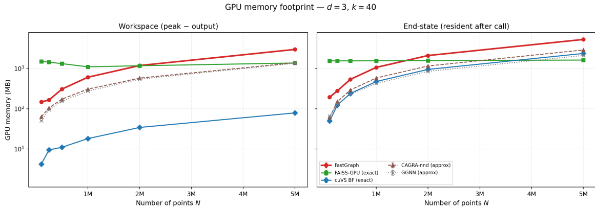
Figure 5: GPU memory footprint per backend at d = 3, k = 40 , measured by a 100 Hz NVML polling thread that captures the true peak during the call. Left : workspace, defined as \text{peak} - N \times k \times (8 + 4) bytes, i.e. everything the algorithm allocates beyond the returned ( idx , dist ) tensors, with idx stored as int64 and dist as float32 ; this isolates temporary algorithm workspace from the common output allocation. Right : end-state, the resident NVML reading after the call synchronises while the caller still holds the output tensors.
