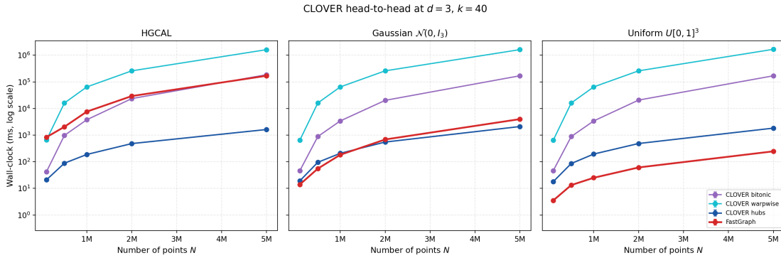
Figure 6: FastGraph vs CLOVER at d=3 , k=40 , across three data distributions: HGCAL recHits (left), synthetic Gaussian N(0, I_3) (center), synthetic uniform on [0, 1]^3 (right). CLOVER’s reference implementation is hardcoded to D=3 at multiple sites ( assert(D == 3) in src/linear-scans.cu ; auto const dim = 3u in include/spatial.cuh ), so d=3 is the only dimensionality at which a direct comparison is possible.
