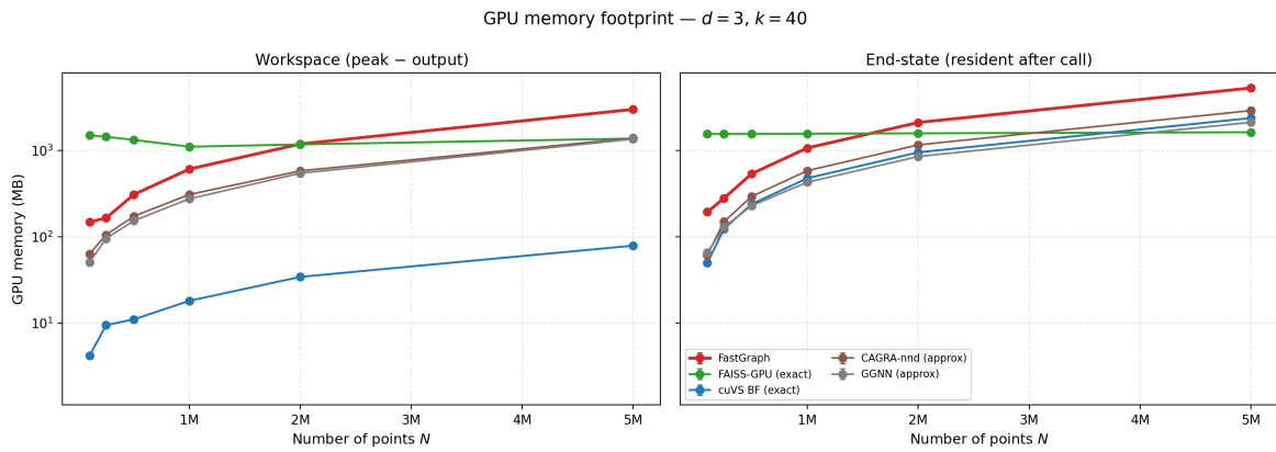
Figure 5: GPU memory footprint per backend at d = 3 , k = 40 , measured by a 100 Hz NVML polling thread that captures the true peak during the call. Left : workspace, defined as peak - (N \times k) output bytes, i.e. everything the algorithm allocates beyond the (idx, dist) output tensors; this isolates temporary algorithm workspace from the common output allocation. Right : end-state, the resident NVML reading after the call synchronises while the caller still holds the output tensors.
