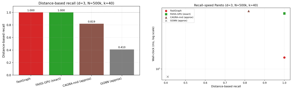
Figure 7: Recall evaluation on HGICAL data. Left : representative distance-based recall at d=3 , N=5 \times 10^5 , k=40 ; FastGraph and FAISS-GPU reach recall = 1.0 under their kernel-matched exact distance conventions. Right : recall-speed Pareto at the same operating point; approximate methods are only competitive when lower recall is acceptable.
