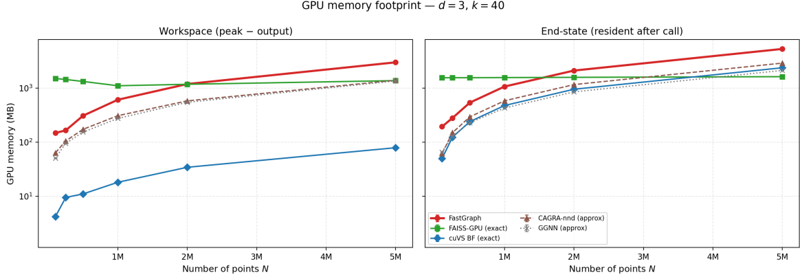
Figure 5: GPU memory footprint per backend at d=3, k=40 , measured by a 100 Hz NVML polling thread that captures the true peak during the call. Left : workspace, defined as peak - N \times k \times (8+4) bytes, i.e. everything the algorithm allocates beyond the returned ( idx , dist ) tensors, with idx stored as int64 and dist as float32 ; this isolates temporary algorithm workspace from the common output allocation. Right : end-state, the resident NVML reading after the call synchronises while the caller still holds the output tensors.
