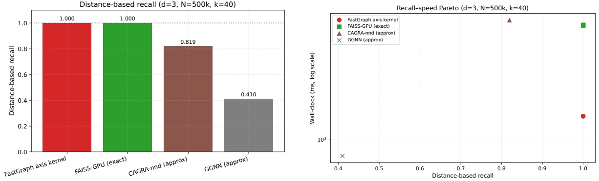
Figure 7: Recall evaluation on HGCAL data. Left : representative distance-based recall at d=3 , N=5 \times 10^5 , k=40 ; the FastGraph axis kernel and FAISS-GPU reach recall = 1.0 under their kernel-matched exact distance conventions. Right : recall-speed Pareto at the same operating point; approximate methods are only competitive when lower recall is acceptable.
