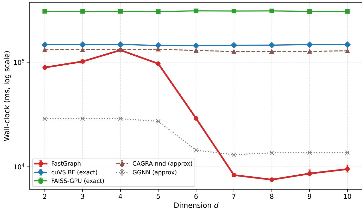
HGCAL kNN graph build — N = 5\text{M} , k = 40
