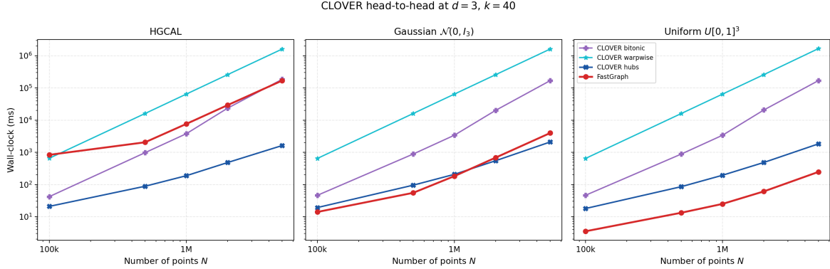
Figure 9: FastGraph vs CLOVER at d=3 , k=40 , across three data distributions: HGICAL recHits (left), synthetic Gaussian \mathcal{N}(0, I_3) (center), synthetic uniform on [0, 1]^3 (right). CLOVER’s reference implementation is hardcoded to D=3 at multiple sites ( assert(D == 3) in src/linear-scans.cu ; auto const dim = 3u in include/spatial.cuh ), so d=3 is the only dimensionality at which a direct comparison is possible.
