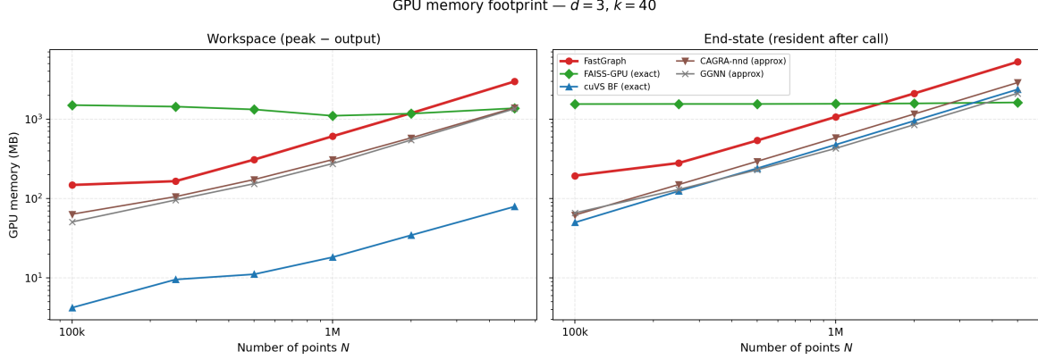
Figure 8: GPU memory footprint per backend at d=3, k=40 , measured by a 100 Hz NVML polling thread that captures the true peak during the call. Left : workspace, defined as peak – (N \times k) output bytes, i.e. everything the algorithm allocates beyond the (\text{idx}, \text{dist}) output tensors. This is the apples-to-apples algorithm-only number. Right : end-state, the resident NVML reading after the call synchronises and the caller still holds the output. This is the “can I fit this in 80 GB” number.
