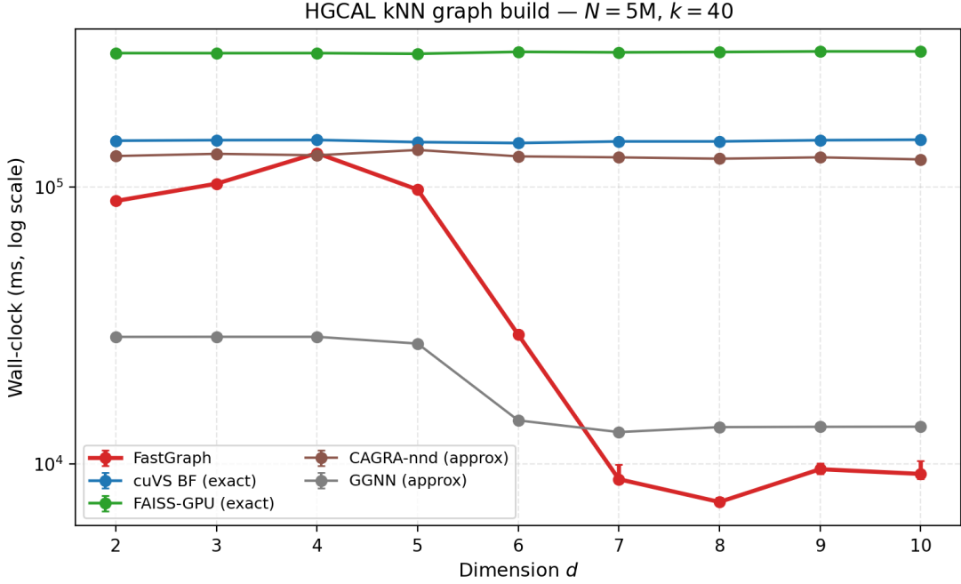
Figure 1: Dimensional scaling on detector data at N=5\text{M} , k=40 . FastGraph is the fastest exact GPU method across the full d=2-10 range. The approximate baseline CAGRA-NN-Descent is included as the strongest approximate GPU comparator; CAGRA’s default IVF-PQ build fails at d \geq 5 on this data (Section 4).
