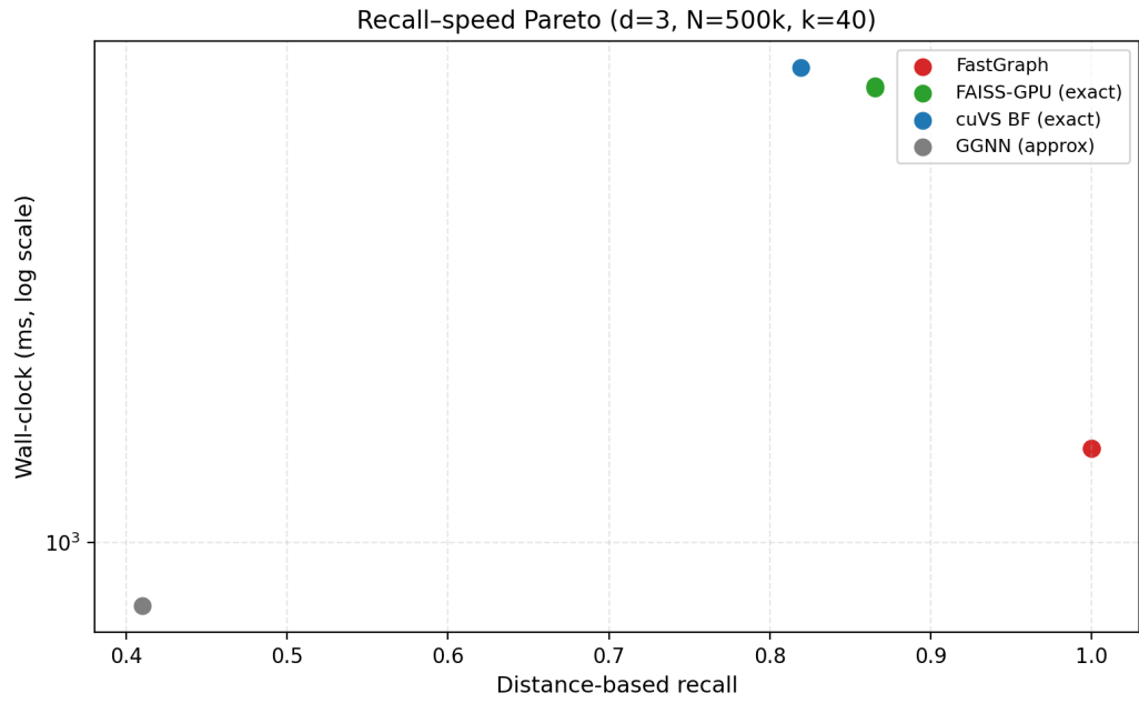
Figure 8: Recall-speed Pareto. FastGraph occupies the exact / fast region; approximate methods are only competitive when lower recall is acceptable.
