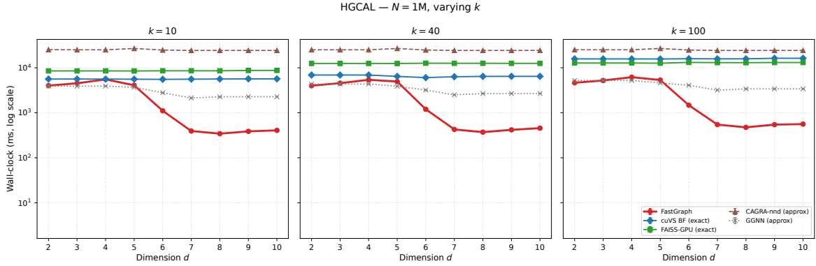
Figure 3: Wall-clock at N=1\text{M} for k \in \{10, 40, 100\} across the full dimensional range. The qualitative pattern of Figure 1 is preserved across k .
