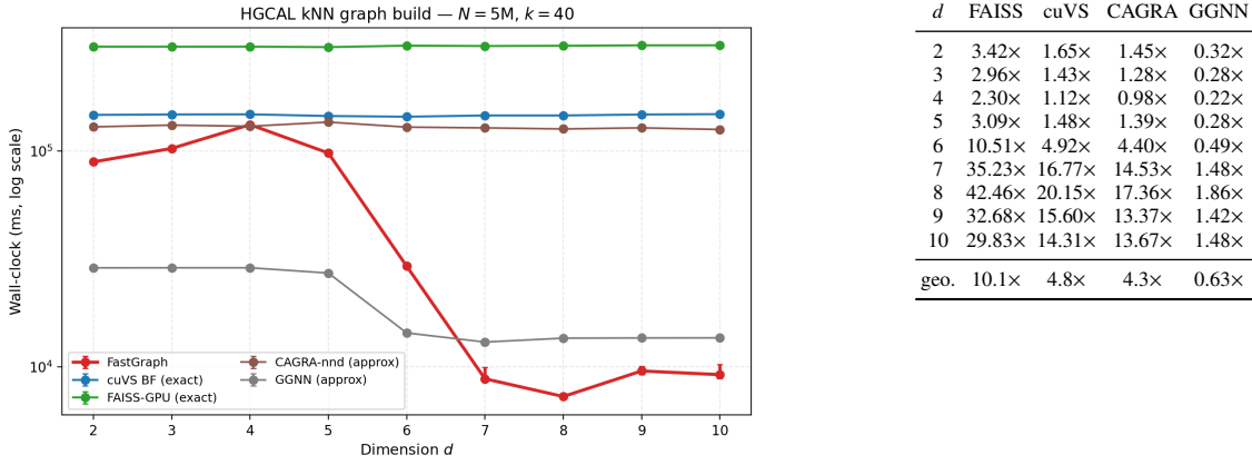
Figure 1: Headline detector benchmark at N=5M, k=40 . Left: dimensional scaling of wall-clock time. FastGraph is the fastest exact GPU method across the full d=2-10 range. Right: speedups of FastGraph over each backend at the same operating point. FAISS and cuVS BF are exact; CAGRA-nnd and GGNN are approximate default-recall baselines, and GGNN’s timing should be read with its substantially lower recall in this regime (Section 5.7).
