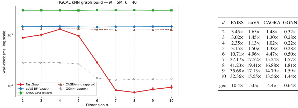
Figure 1: Headline benchmark on detector data at N=5M , k=40 . Left: dimensional scaling of wall-clock time. FastGraph is the fastest among the tested dimension-general exact GPU baselines across the full d=2-10 range. Right: speedups of FastGraph over each backend at the same operating point. FAISS and cuVS BF are exact; CAGRA-nnd and GGNN are approximate default-recall baselines, and GGNN’s timing should be read with its substantially lower recall in this regime (Section 5.7).
