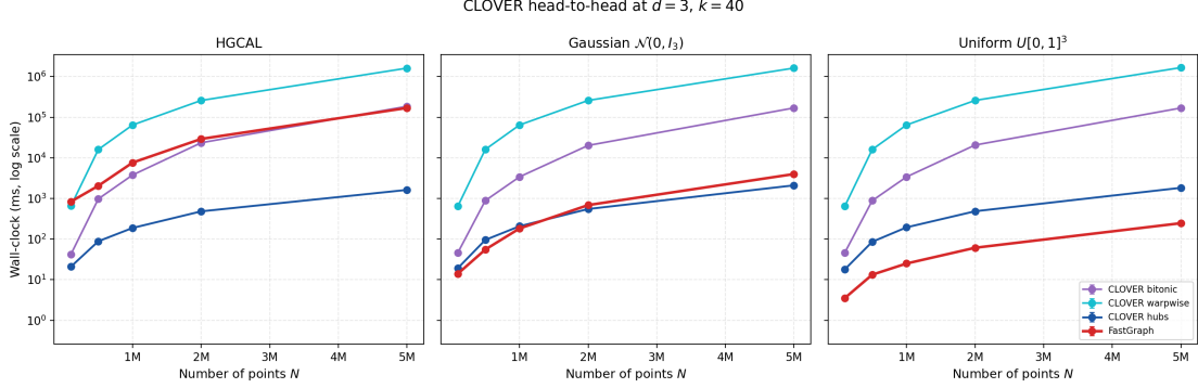
Figure 6: FastGraph vs CLOVER at d=3 , k=40 , across three data distributions: HGICAL recHits (left), synthetic Gaussian \mathcal{N}(0, I_3) (center), synthetic uniform on [0, 1]^3 (right). CLOVER’s reference implementation is hardcoded to D=3 at multiple sites ( assert(D == 3) in src/linear-scans.cu ; auto const dim = 3u in include/spatial.cuh ), so d=3 is the only dimensionality at which a direct comparison is possible.
