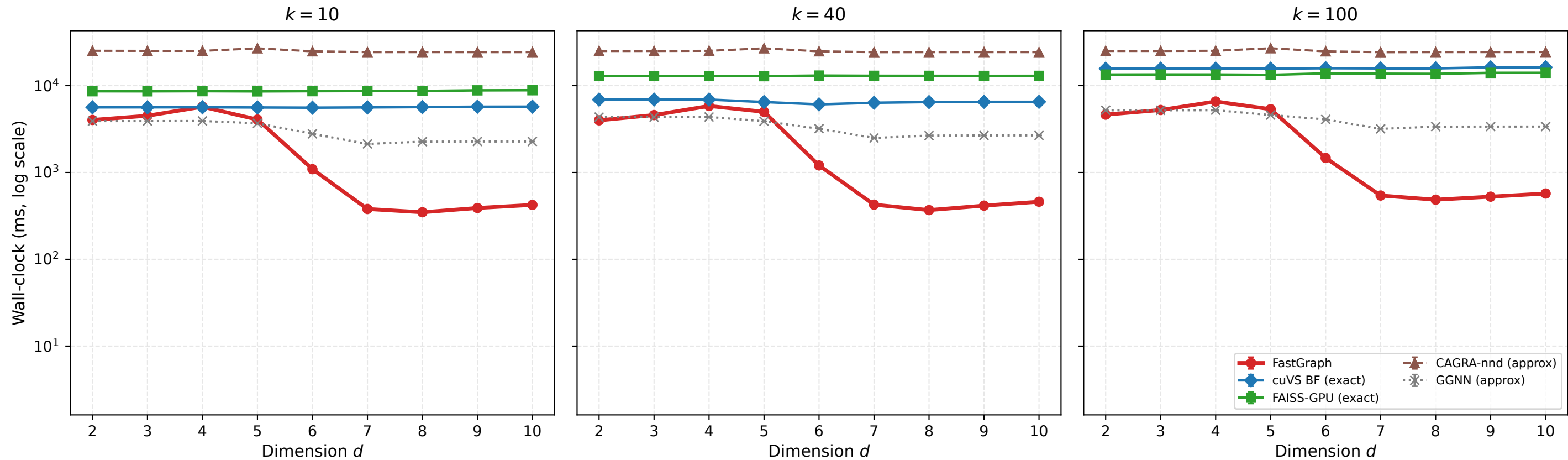
HGCAL — N = 1\text{M} , varying k
