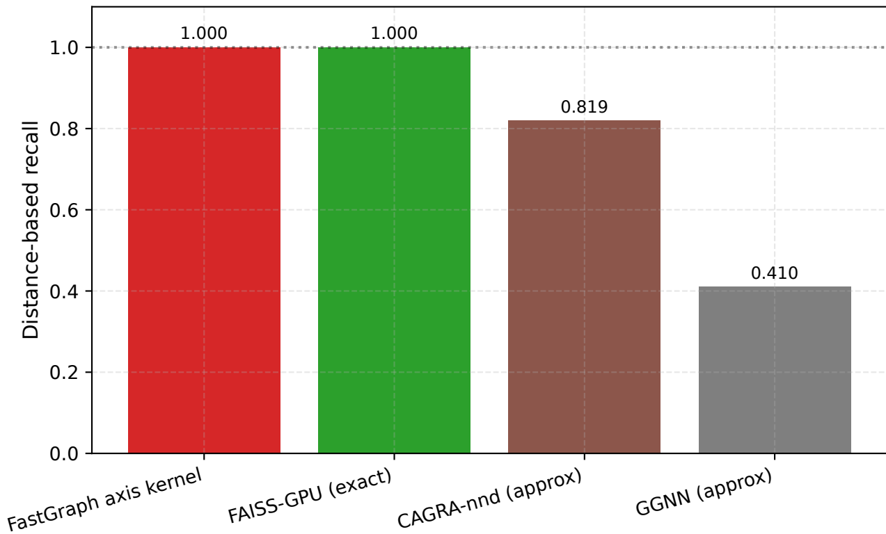
Distance-based recall ( d=3 , N=500k , k=40 )
