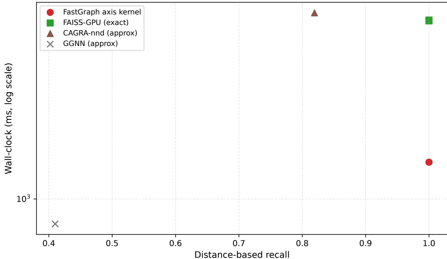
Recall-speed Pareto (d=3, N=500k, k=40)
