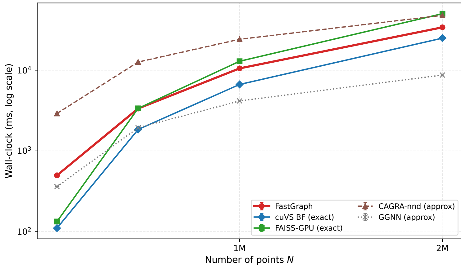
Isotropic Gaussian — d = 8, k = 40
