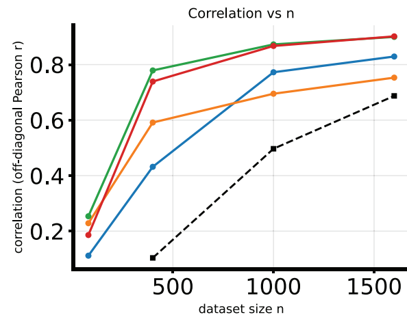
Non-fourier input
