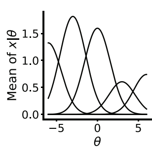
Non-fourier input
