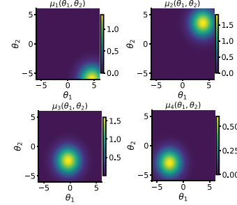
Non-fourier input
