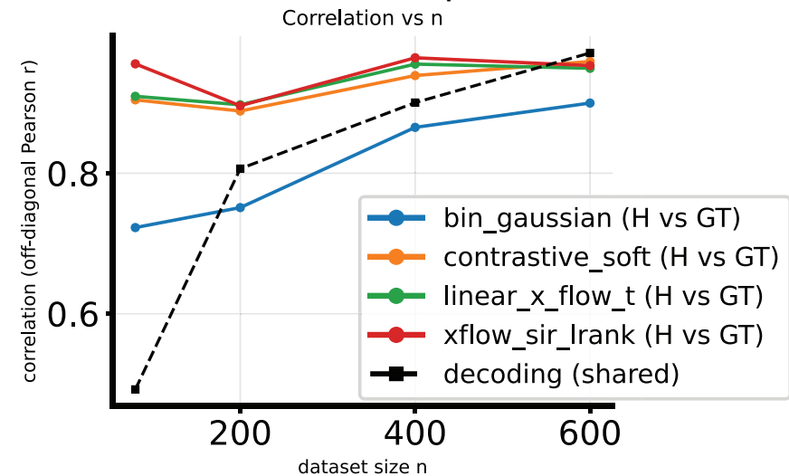
Non-fourier input
