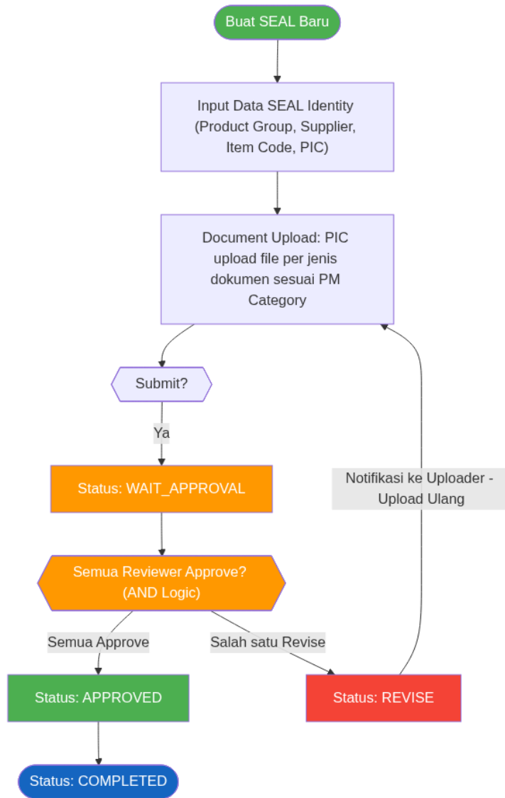
SEAL Business Flow Diagram
