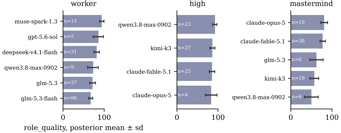
Figure 6: The seed index shipped in the binary: 15 cells from 190 scored runs, \text{role\_quality} = 100 \cdot P(\text{no major defect}) under a \text{Beta}(1,1) posterior. The spread between models a catalog rates alike is why the pool exists.
