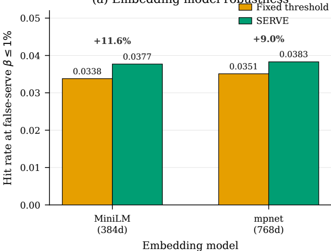
(a) Embedding model robustness
