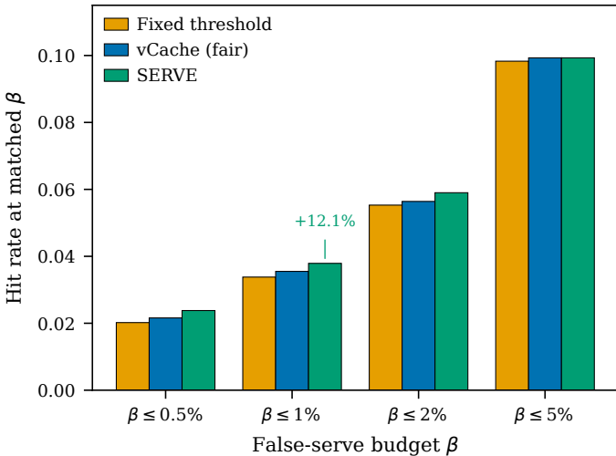
(a) Hit rate vs. false-serve budget \beta
