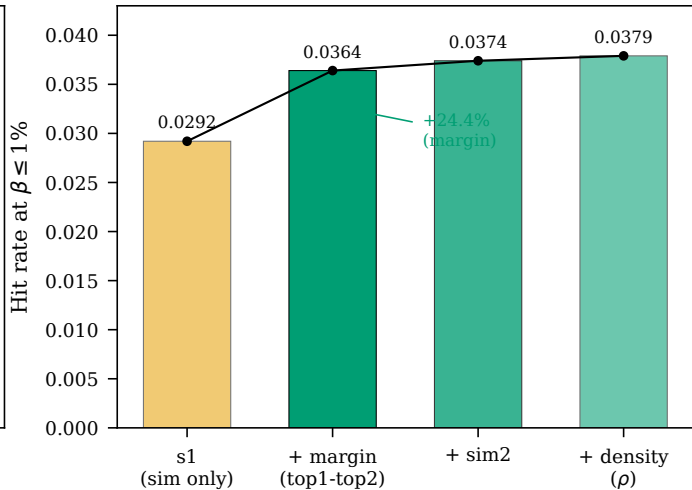
(b) Cumulative feature ablation ( \beta \leq 1\% )
