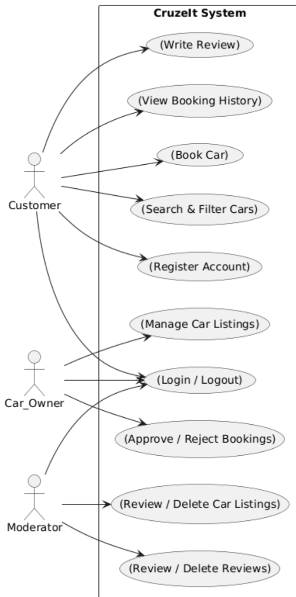
Figure 4 - Use Case Diagram of the CruzeIt System
