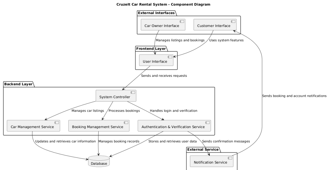
Figure 3 - Component Diagram of the CruzeIt Architecture
