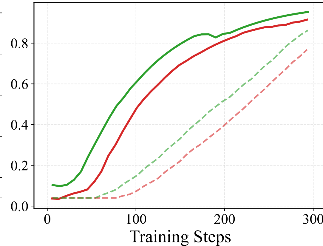
AlgorithmScheduling
