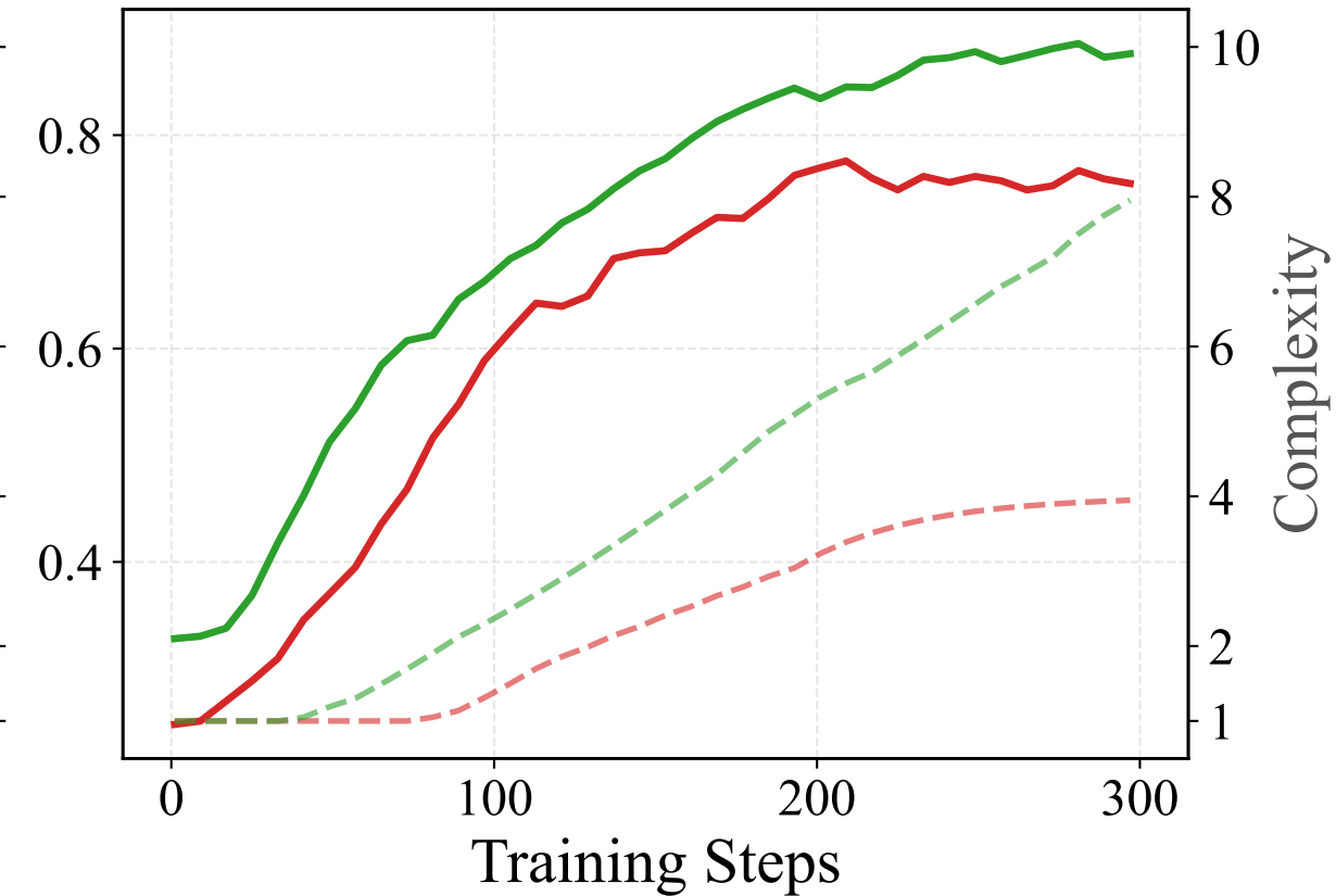
RunicPotionGame
