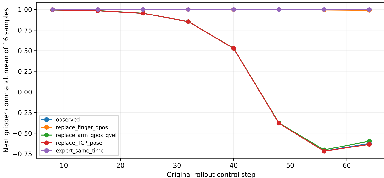
Paired-noise input probe: finger position drives the premature closure
