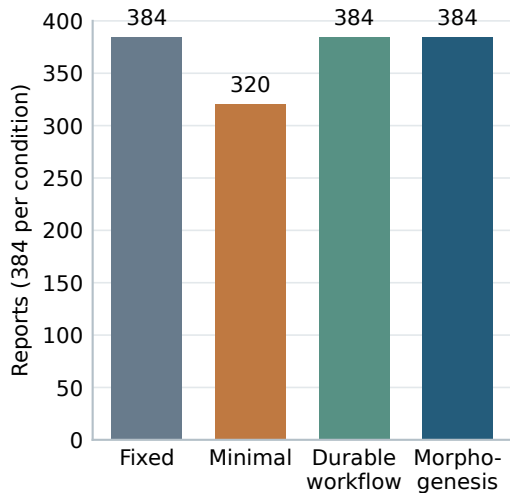
Correct final reports
