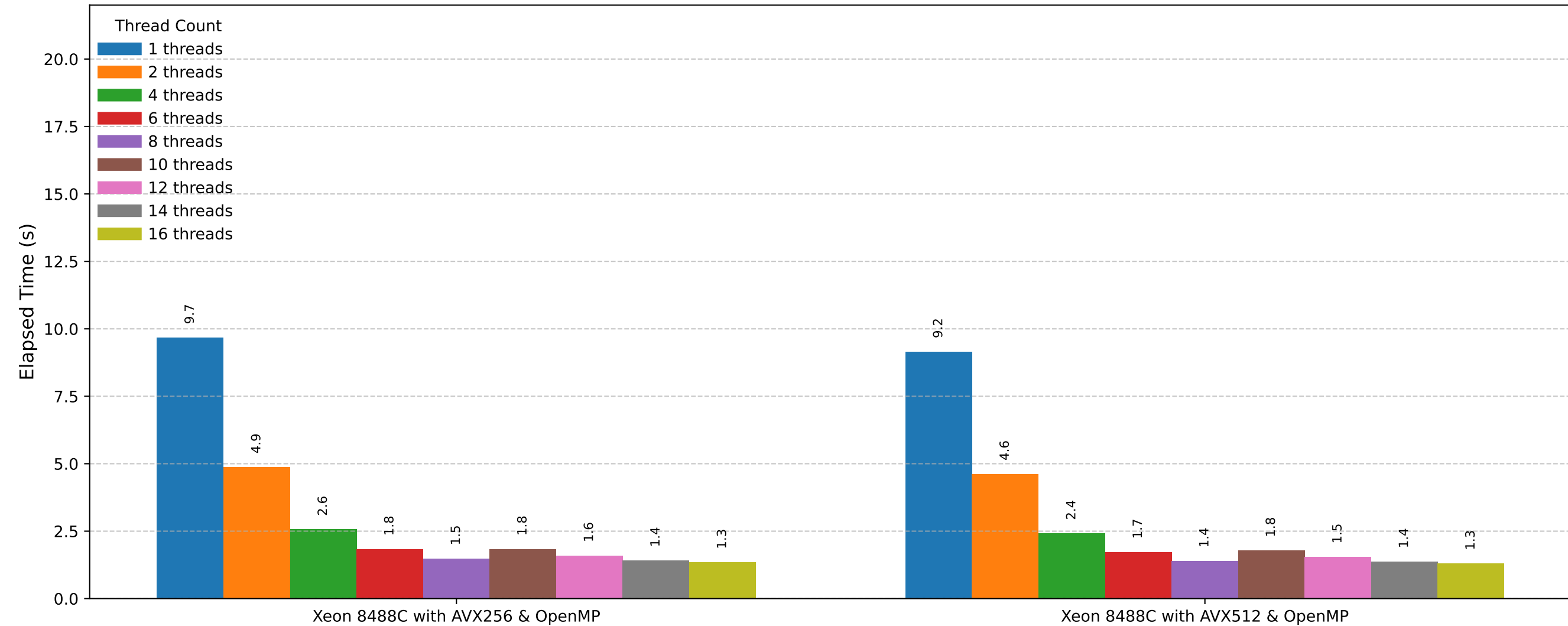
Threads Performance Evaluation on Xeon 8488C
