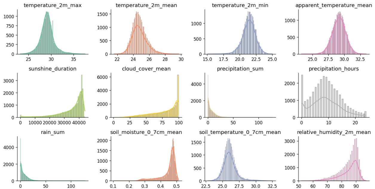
Gambar 1: Distribusi Variabel
