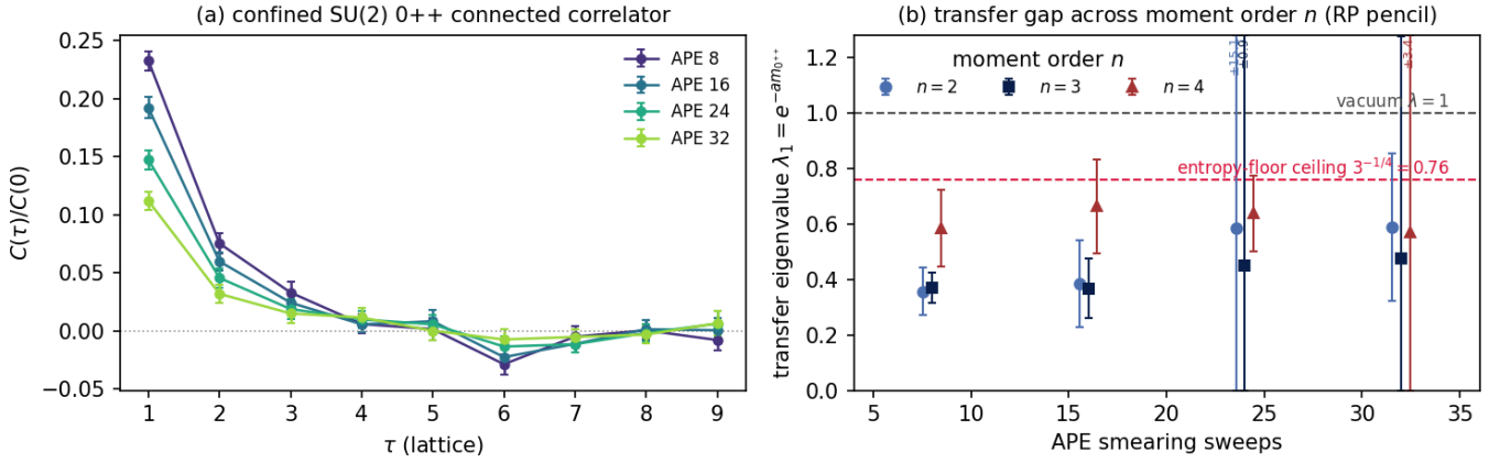
Figure 7. The transfer gap on confined SU(2) ( \beta = 2.30 , L = 16^3 \times 28 , 512 configurations). (a) The APE-smear 0^{++} connected correlator C(\tau)/C(0) (jackknife errors, four smearing levels): positive and decaying out to \tau = 5 , in noise beyond, so the moment matrix is reflection-positive on the resolved lags. (b) The reflection-positive moment-pencil transfer eigenvalue \lambda_1 = e^{-a m_{0^{++}}} against smearing, at every moment order n \in \{2, 3, 4\} (true jackknife bars; oversized bars at heavy smearing are labelled, not clipped): the leading mode sits below the vacuum \lambda = 1 , with n=2, 3 isolated at \approx 0.35\text{--}0.38 under the entropy-floor ceiling 3^{-1/4} = 0.76 and n=4 the moment-order systematic at \approx 0.6 — the §13 isolated-mode hypothesis, measured, with its systematic shown.
