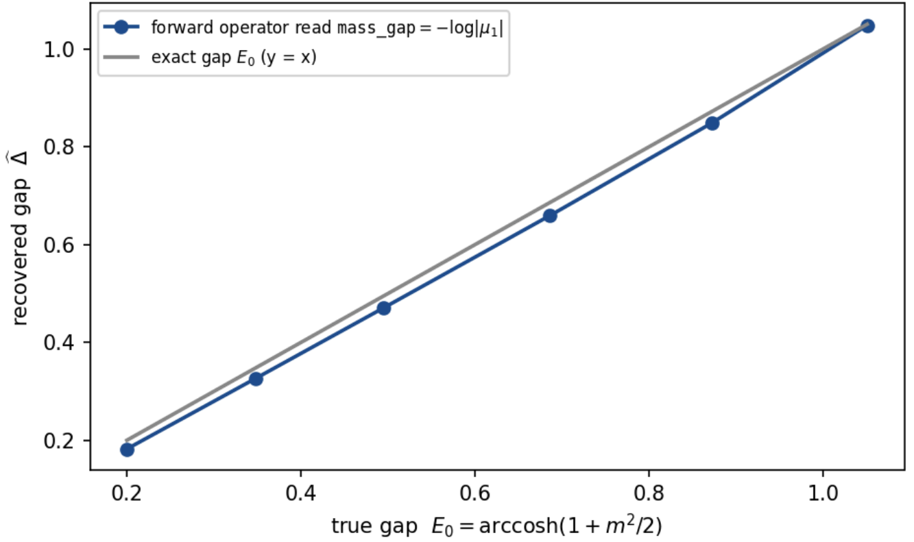
Figure 4. The free-scalar gap calibration. The DMD/Koopman operator read, a forward operator identification reading -\log |m_1| off the trajectory, recovers the exact gap E_0 = \text{arccosh}(1 + m^2/2) across m \in [0.20, 1.10] , the finite temporal extent setting the approach (8.9% at m = 0.20 to 0.2% at m = 1.10 as \xi/L_t shrinks). It certifies the read as a gap instrument on the one field that carries its gap directly.
