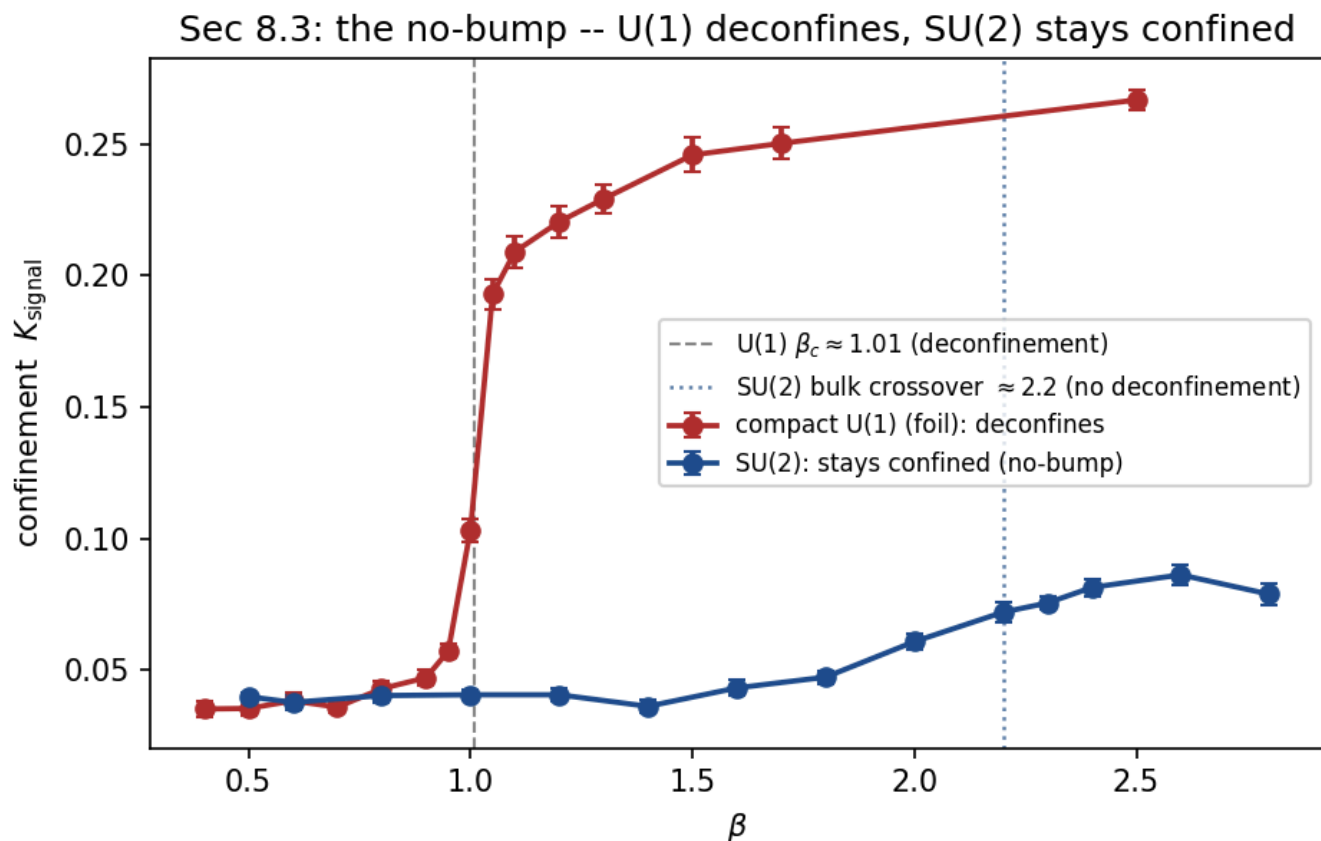
Figure 1. The no-bump. Across \beta = 0.4 – 2.8 the confinement order parameter K_{\text{signal}} stays flat and low for SU(2) (confined at every coupling, 0.04 – 0.09 ), while compact U(1) steps sharply up past its deconfinement transition \beta_c \approx 1.011 ( 0.04 \rightarrow 0.27 ). Read on raw configurations, pinned to the confined-vacuum null, no fit.
