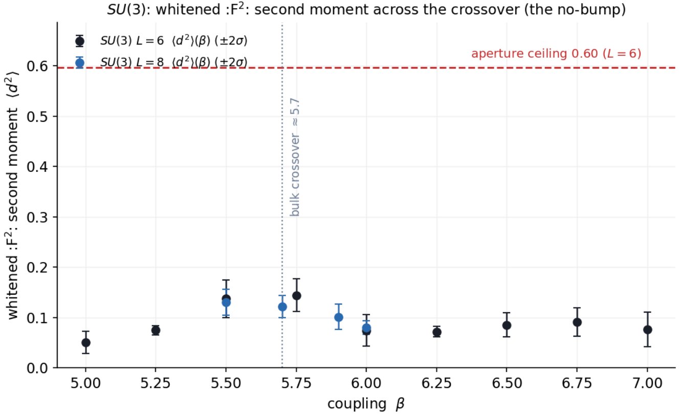
Figure 12. The same interior read on SU(3) . The whitened :F^2: second moment \langle d^2 \rangle(\beta) read on pure- SU(3) L=6, 8 configurations (same direct-lag read, \pm 2\sigma bootstrap) stays \in [0.05, 0.15] across \beta = 5.0-7.0 , a factor \gtrsim 4 below its aperture ceiling (0.60 at L = 6 , red dashed), passing the bulk crossover near \beta \approx 5.7 with no bump. The finite-correlation-length interior read holds on a second gauge group.
