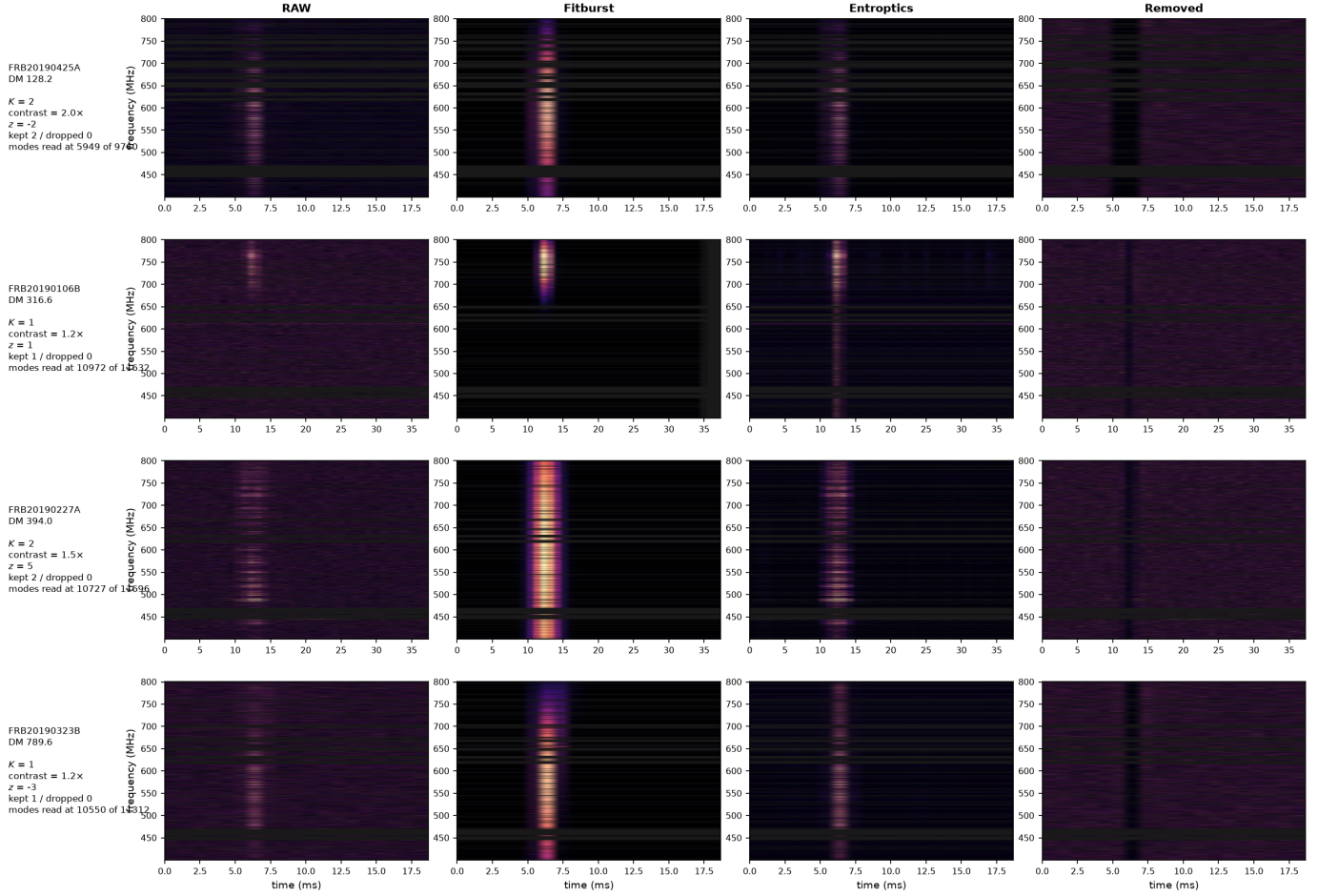
Real CHIME/FRB bursts, read untuned: raw = Entropitics + Removed
