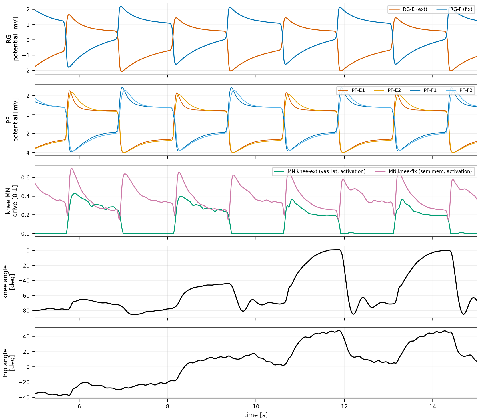
gait2392 spinal SNS - right leg (ground_pose, RoM limits + Renshaw 0.5)
