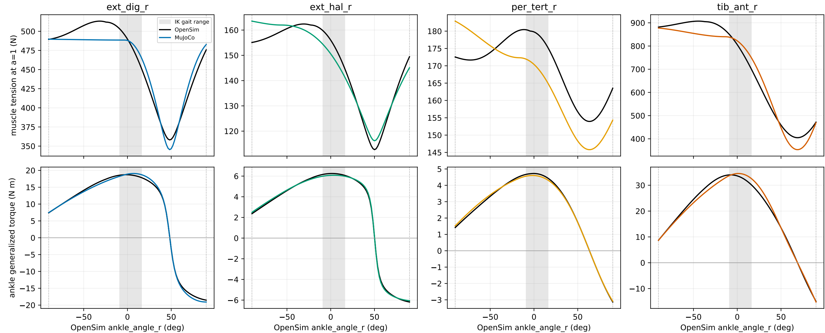
Right ankle dorsiflexor capacity: OpenSim reference vs converted MuJoCo shading = measured IK gait range; dotted = MuJoCo joint limits
