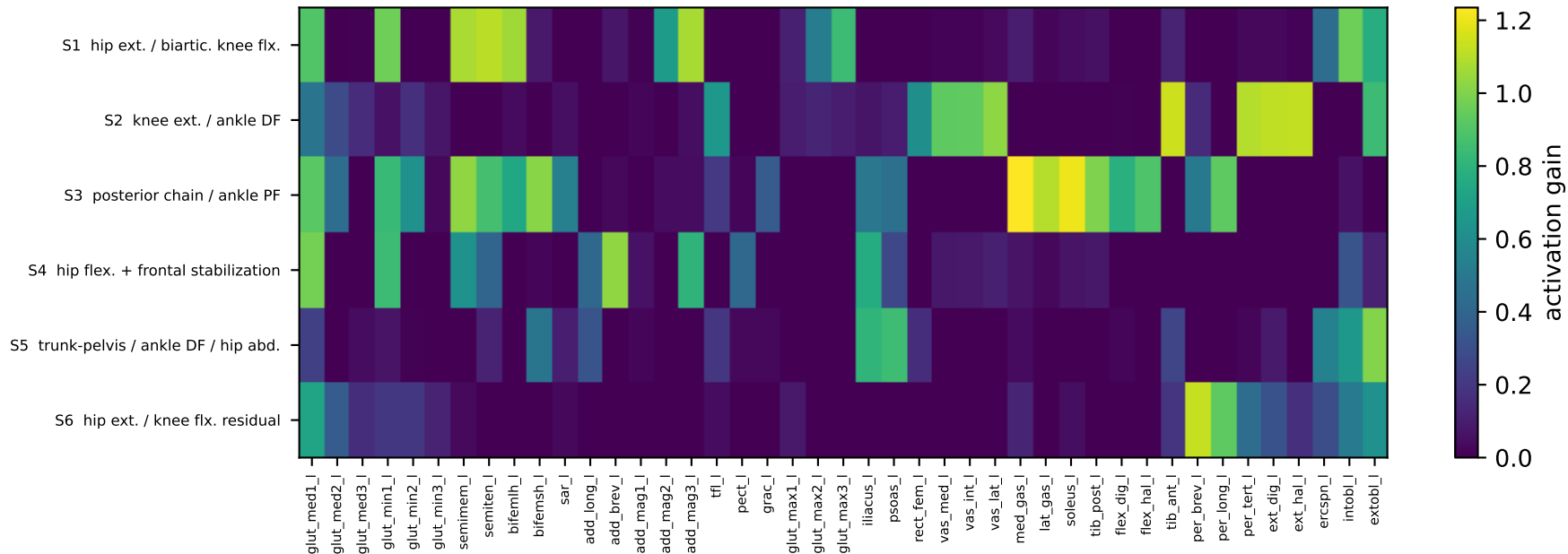
NMF spatial gains (extracted synergies; functional labels provisional)
