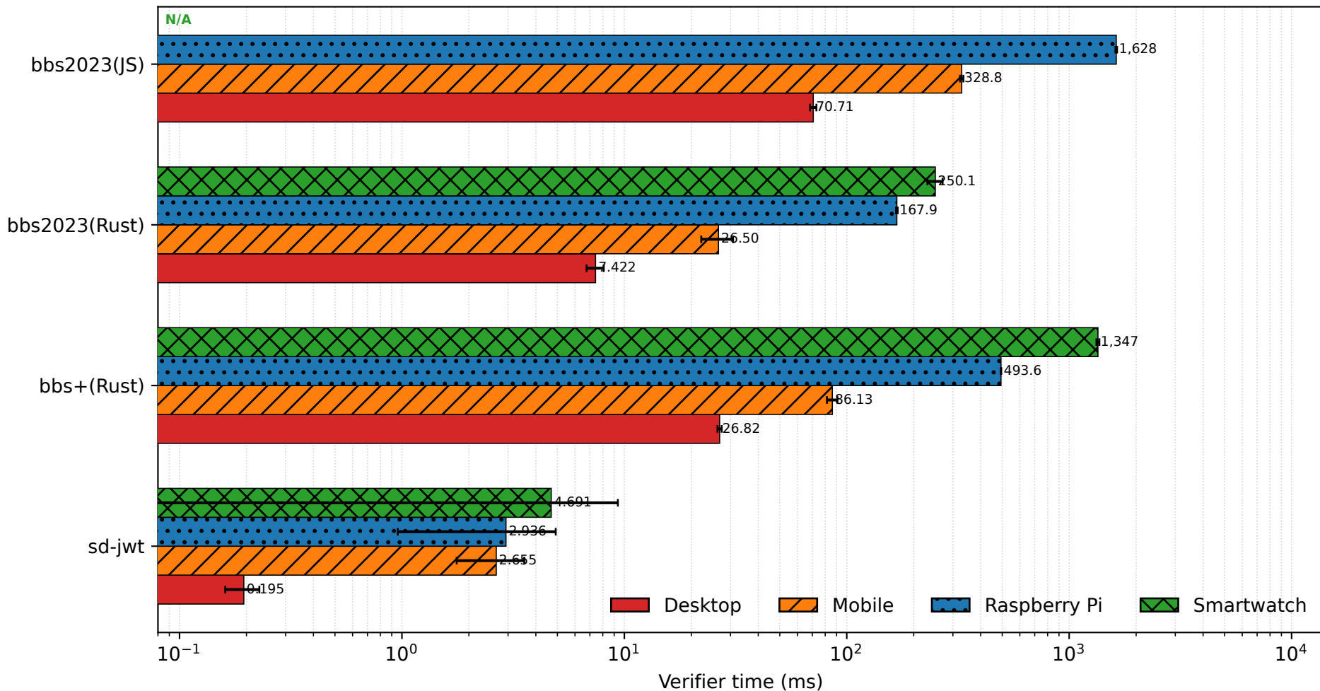
Verifier time Slice: reveal=0.80, attrCount=7
