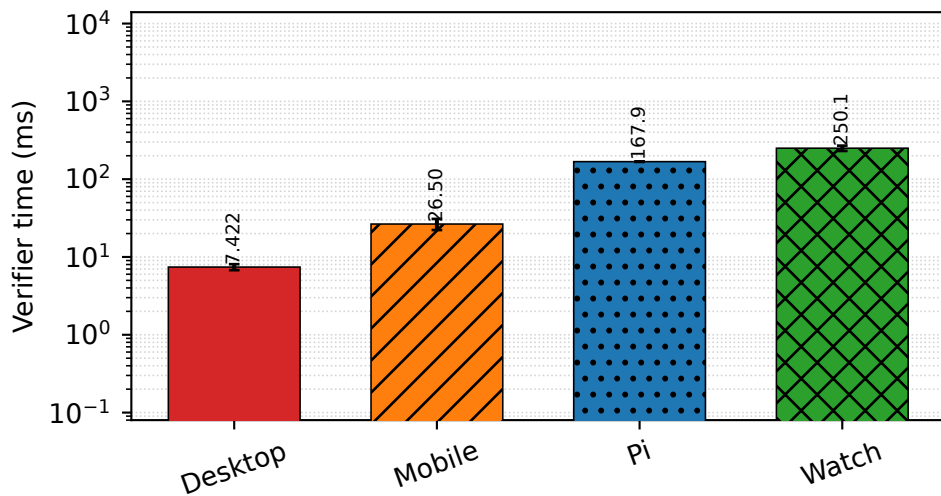
bbs2023(Rust)
