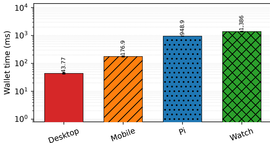
bbs2023(Rust)
