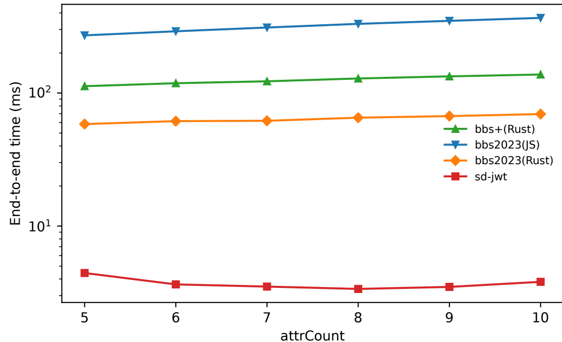
End-to-end time (ms) vs AttrCount
