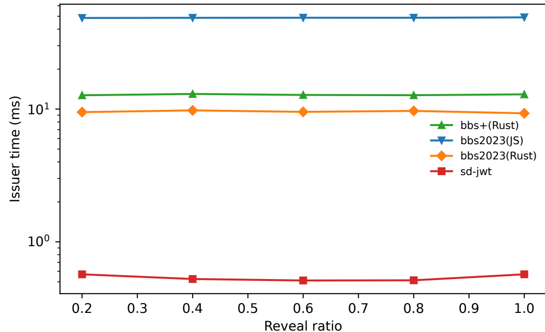
Issuer time (ms) vs Reveal
