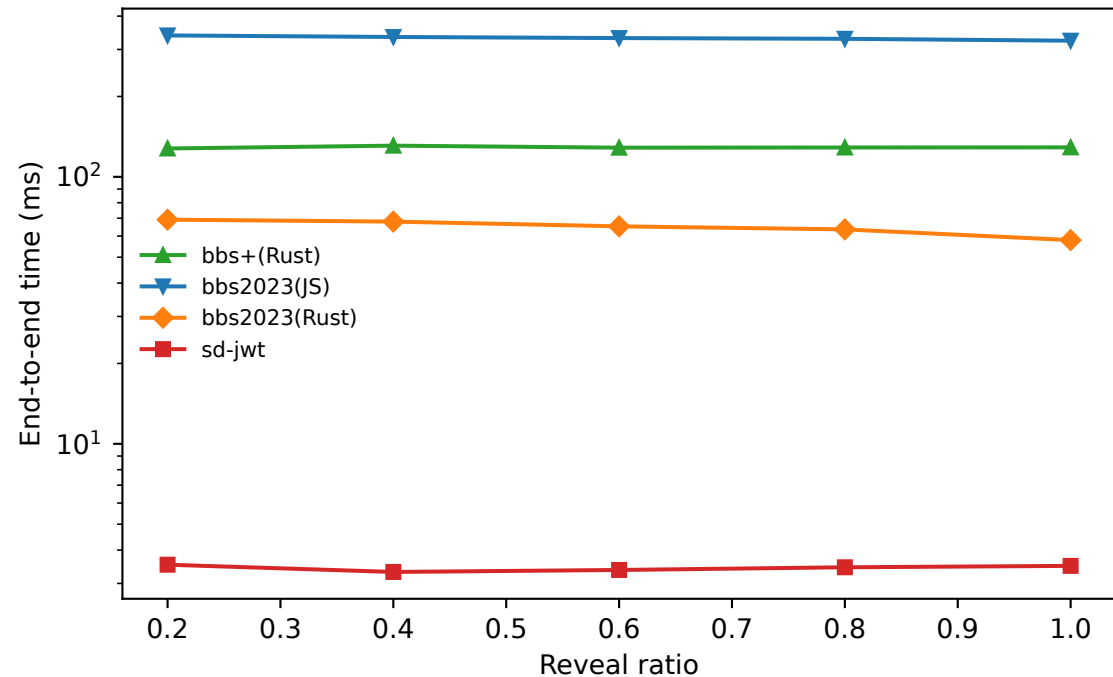
End-to-end time (ms) vs Reveal
