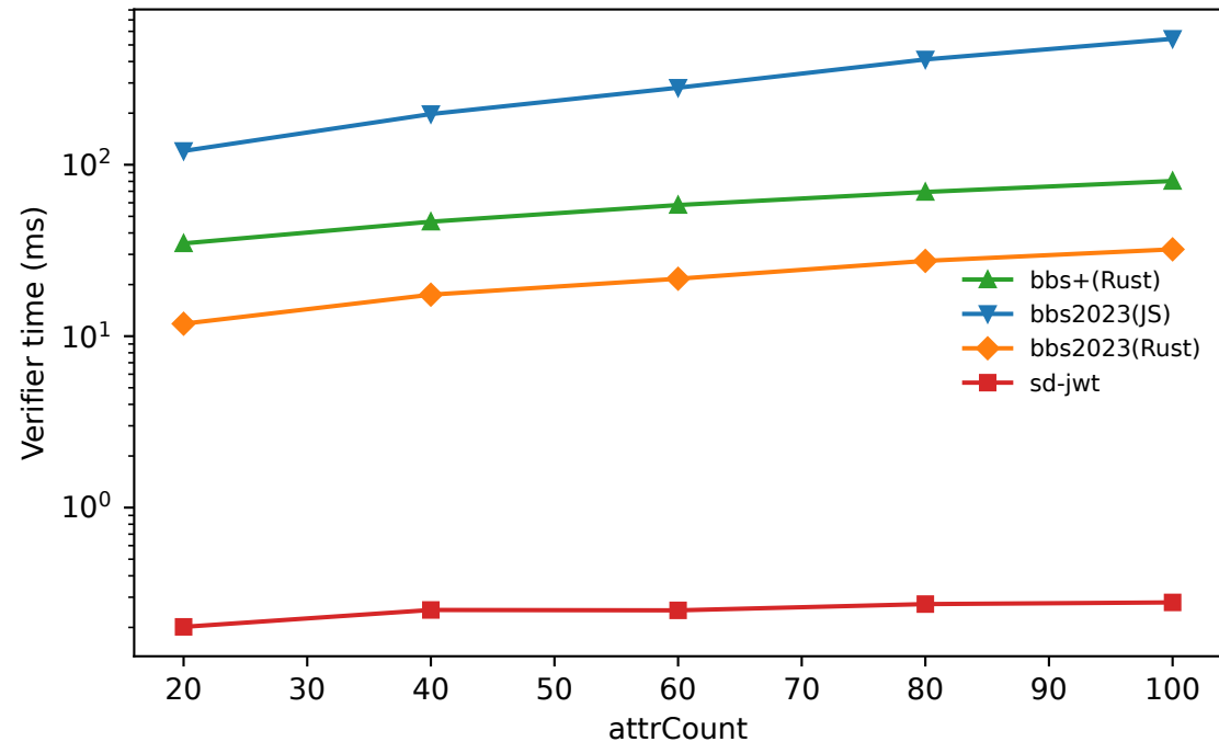
Verifier time (ms) vs AttrCount
