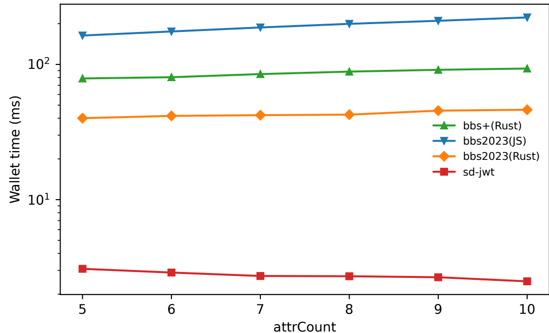
Wallet time (ms) vs AttrCount
