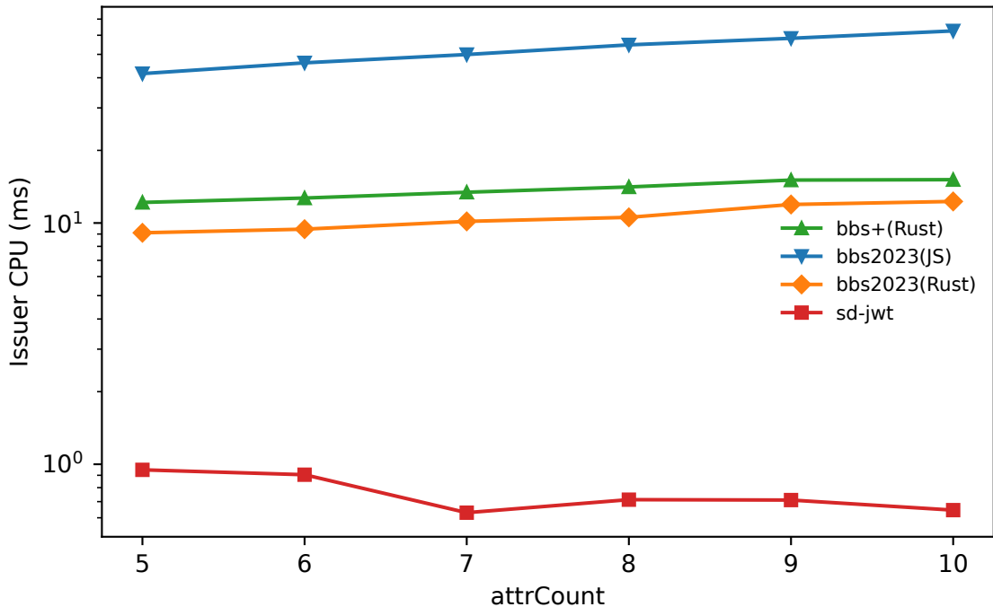
Issuer CPU (ms) vs AttrCount
