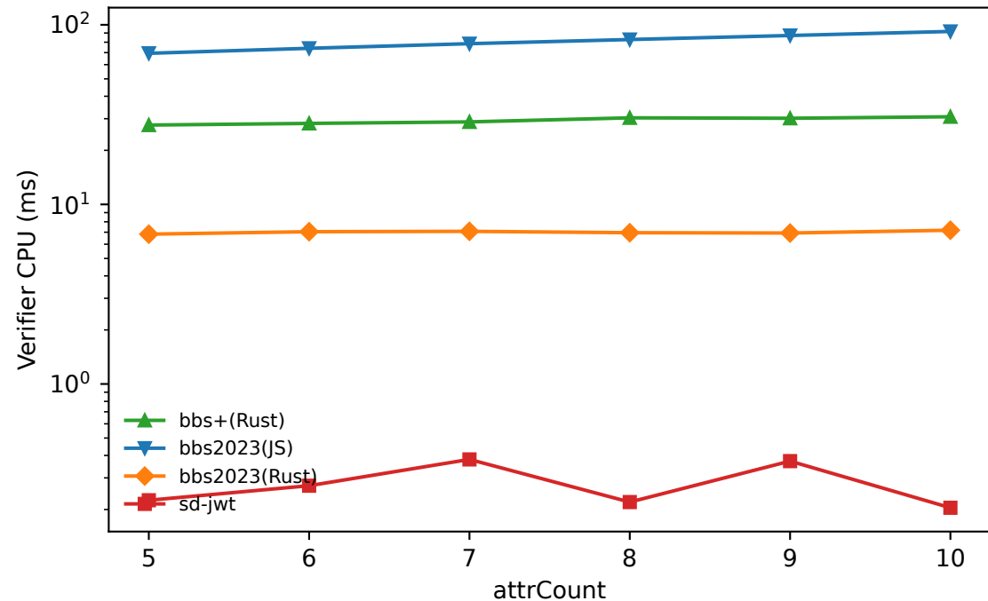
Verifier CPU (ms) vs AttrCount
