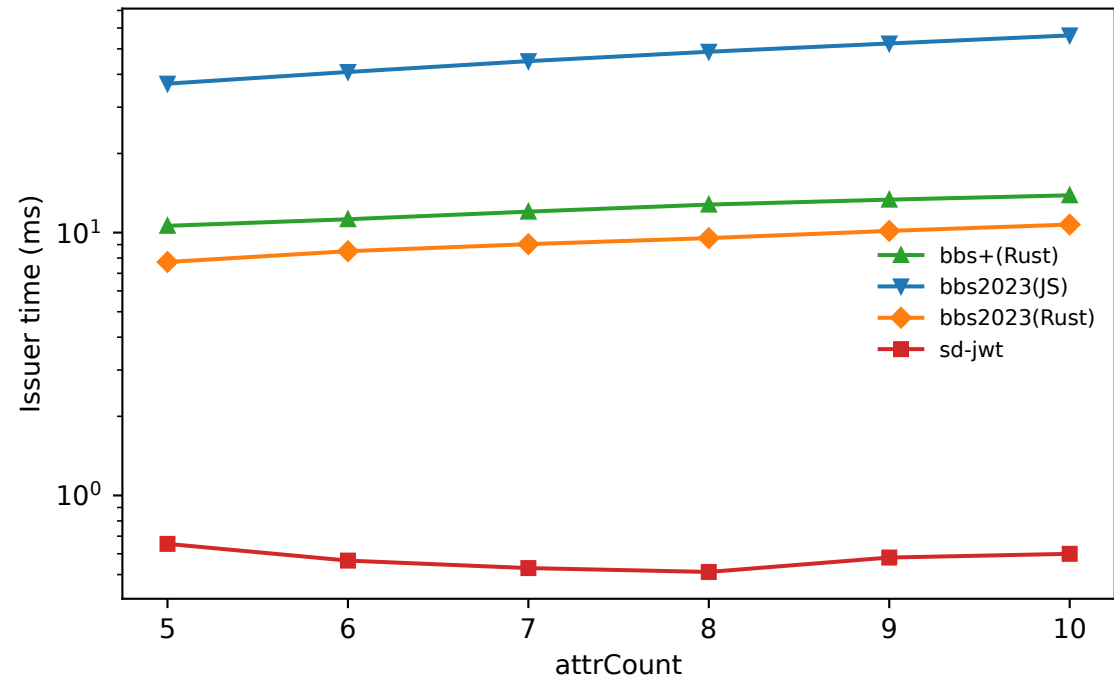
Issuer time (ms) vs AttrCount
