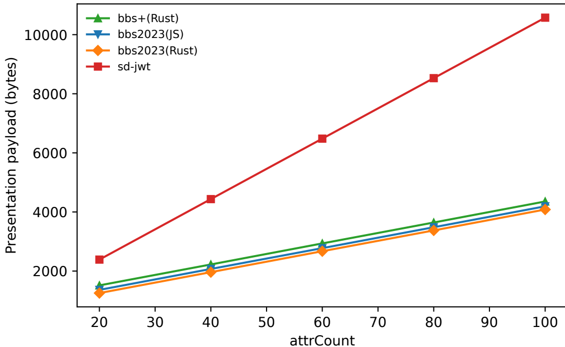
Presentation payload (bytes) vs AttrCount
