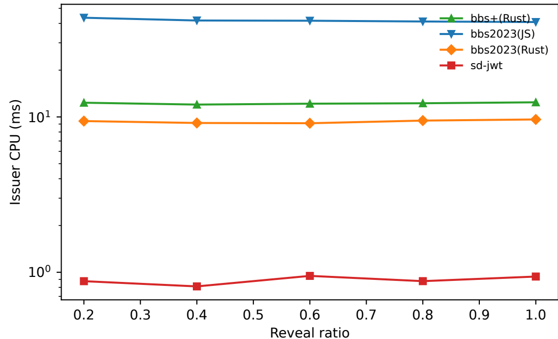
Issuer CPU (ms) vs Reveal
