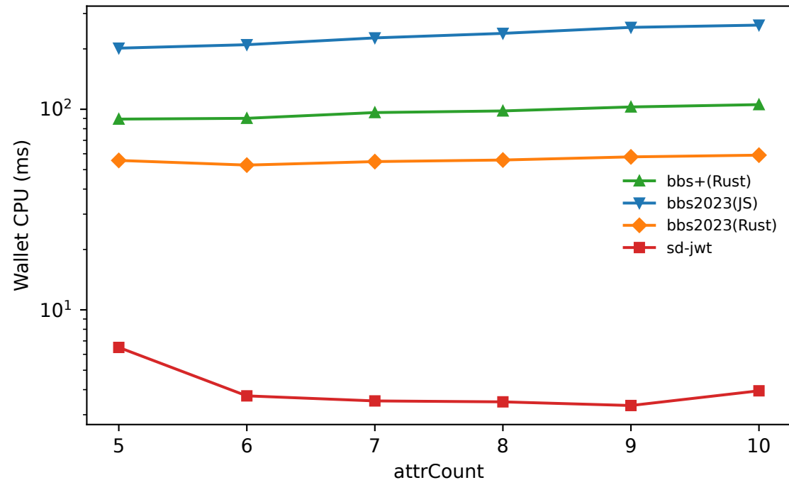
Wallet CPU (ms) vs AttrCount
