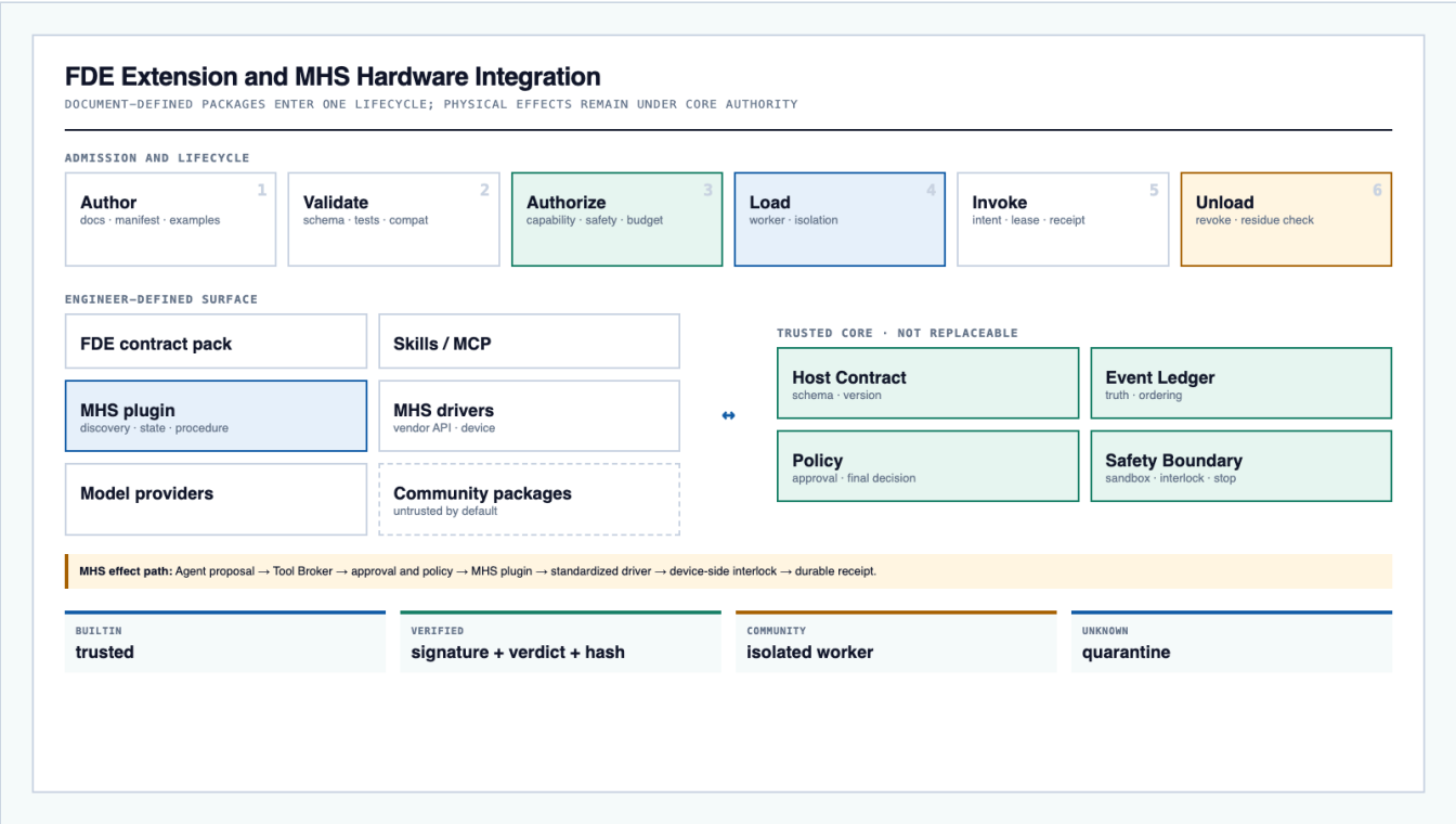
Figure 9. FDE-authored packages and MHS device drivers enter through one governed lifecycle. Capability expansion is open, while protocol truth, effect authorization, and physical safety boundaries remain closed to replacement.
