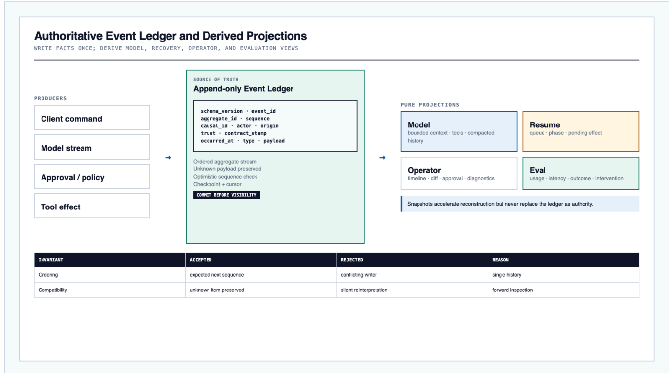
Figure 6. One ordered event stream produces four consumer-specific views. This avoids separate, drifting histories for the model, UI, recovery, and evaluation.
