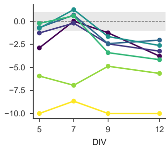
f Burst rate
