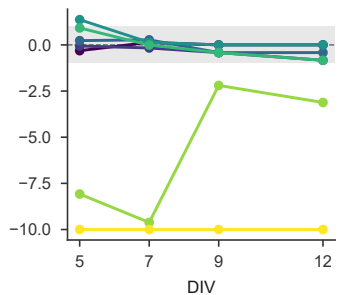
c Bursting electrodes
