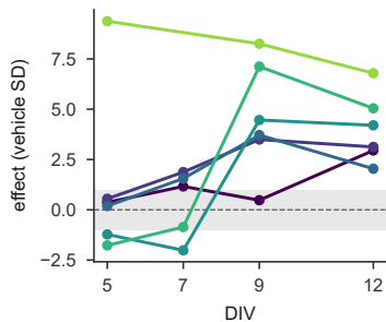
d Inter-NS interval
