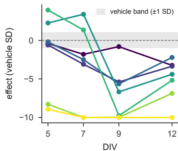
a Network spikes (NS)
