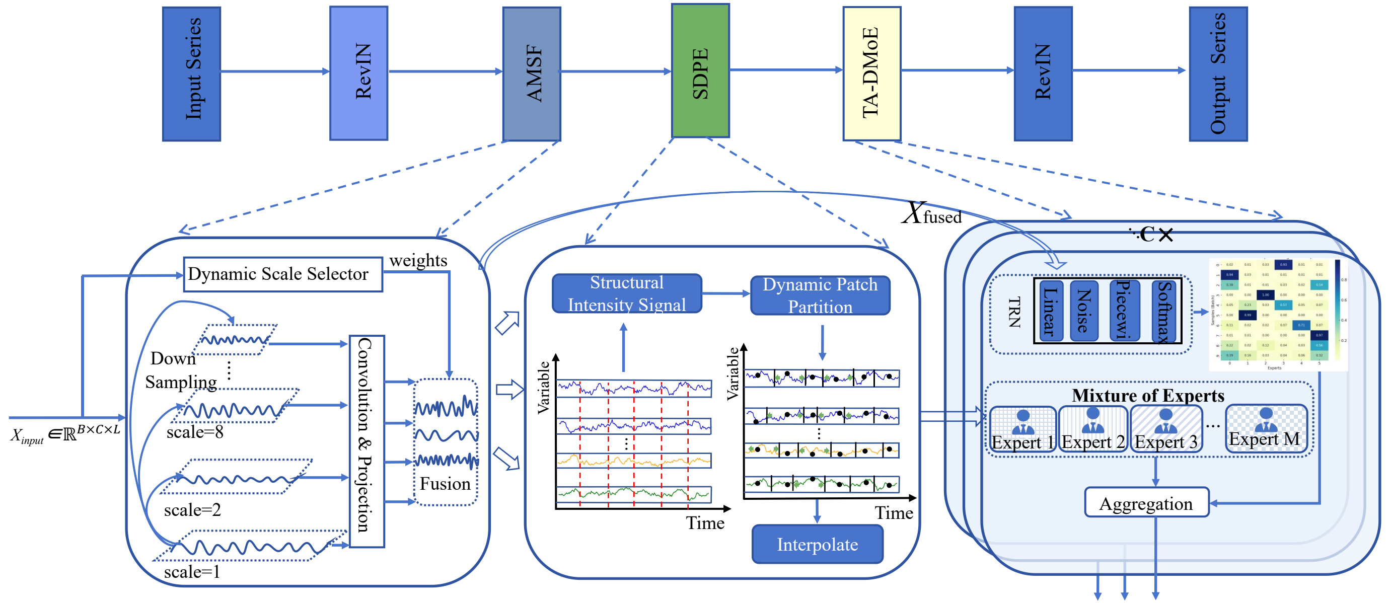
(a). Adaptive Multi-Scale Fusion
