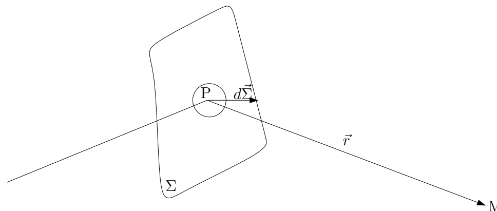
FIGURE 1.2 – Principe de Huygens-Fresnel.
