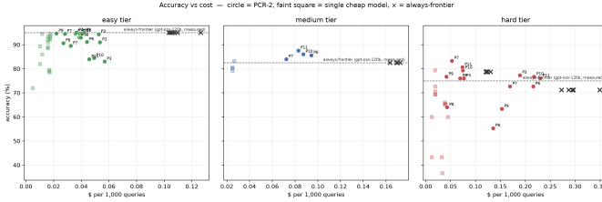
Fig. 2. Accuracy vs. cost per 1,000 queries. Circles = PCR-2, faint squares = single cheap model, × = Always-Frontier (gpt-oss-120b, measured), dashed line = its accuracy. Easy tier: PCR-2 within \approx 1 pp of frontier accuracy at \approx 1/3 the cost.
