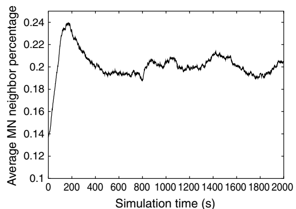
Fig. 4. Average neighbor percentage versus time.
