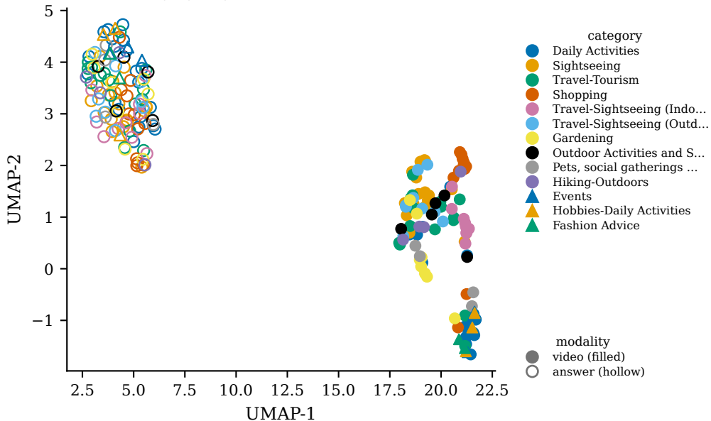
Shared SigLIP space: video vs. answer, colored by category google/siglip2-so400m-patch14-384
