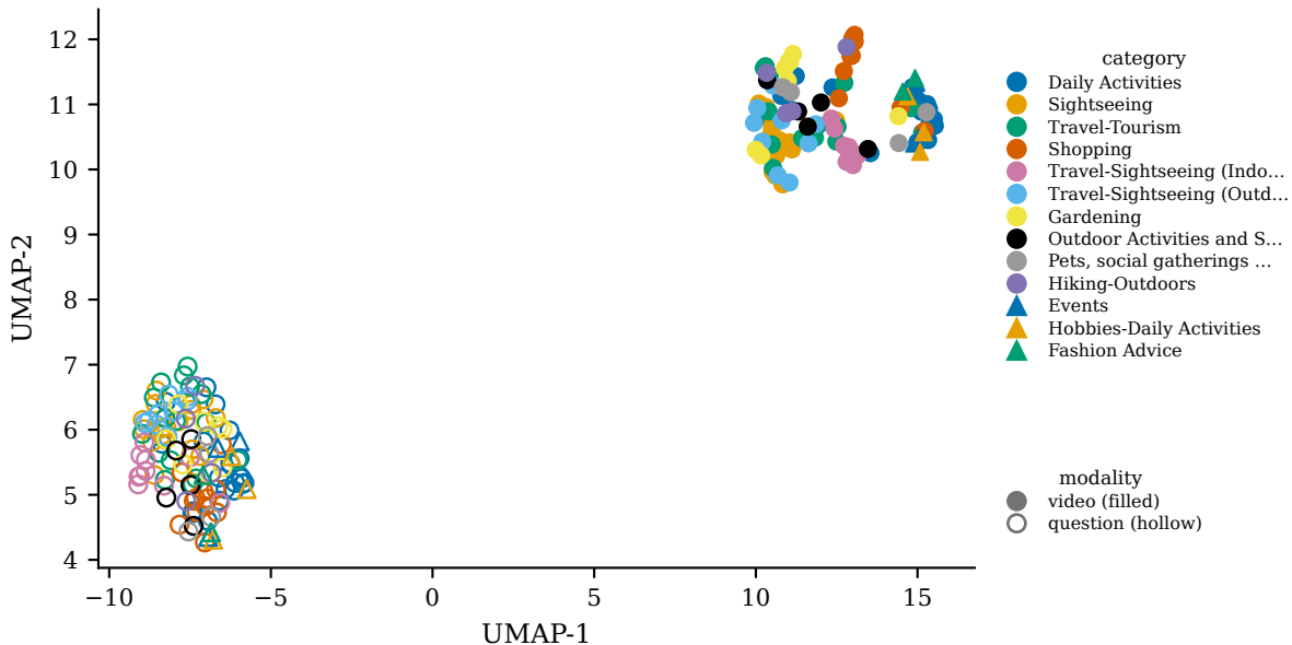
Shared SigLIP space: video vs. question, colored by category google/siglip2-so400m-patch14-384
